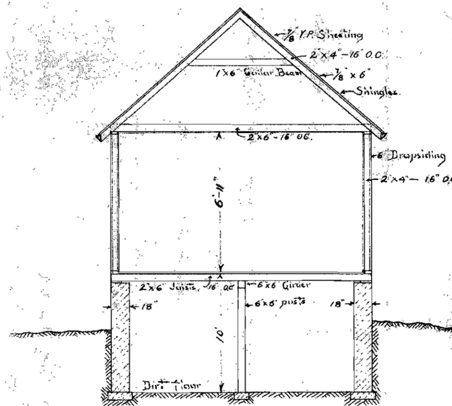
CROSS-SECTION
