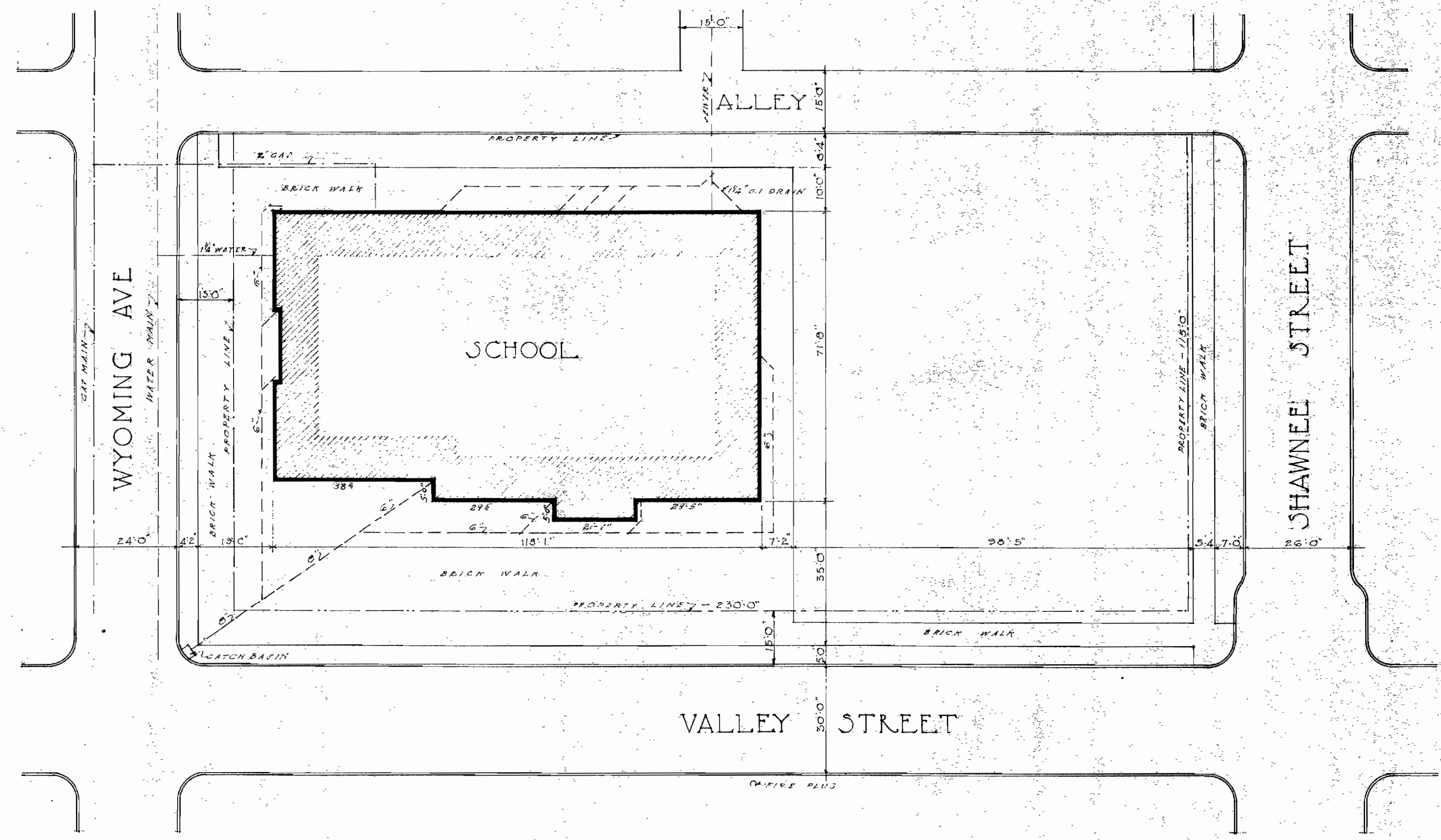
PLOT PLAN SCALE 0 5 10 15 20 30
