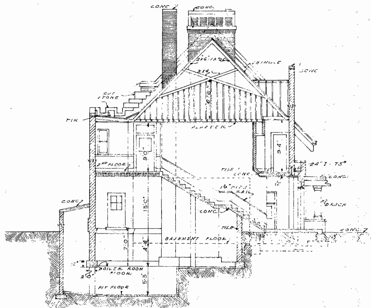
CROSS SECTION
