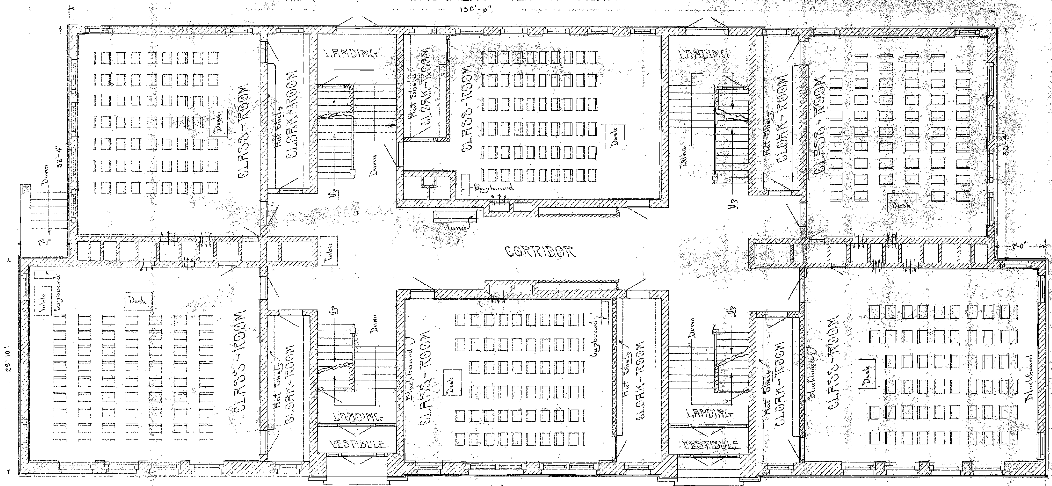
FIRST - FLOOR - PLAN 144'-6"
