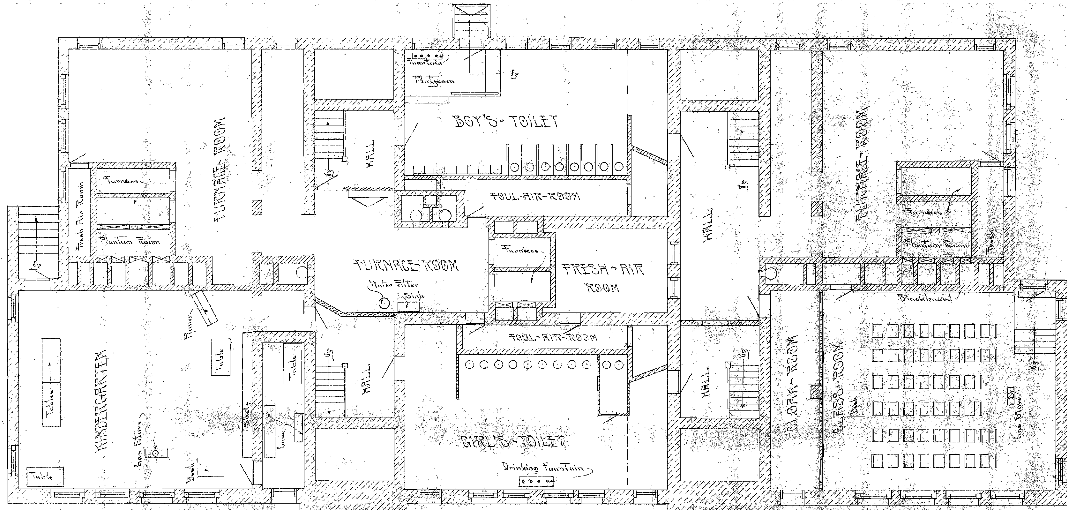
BASEMENT - FLOOR - PLAN 130'-6"
