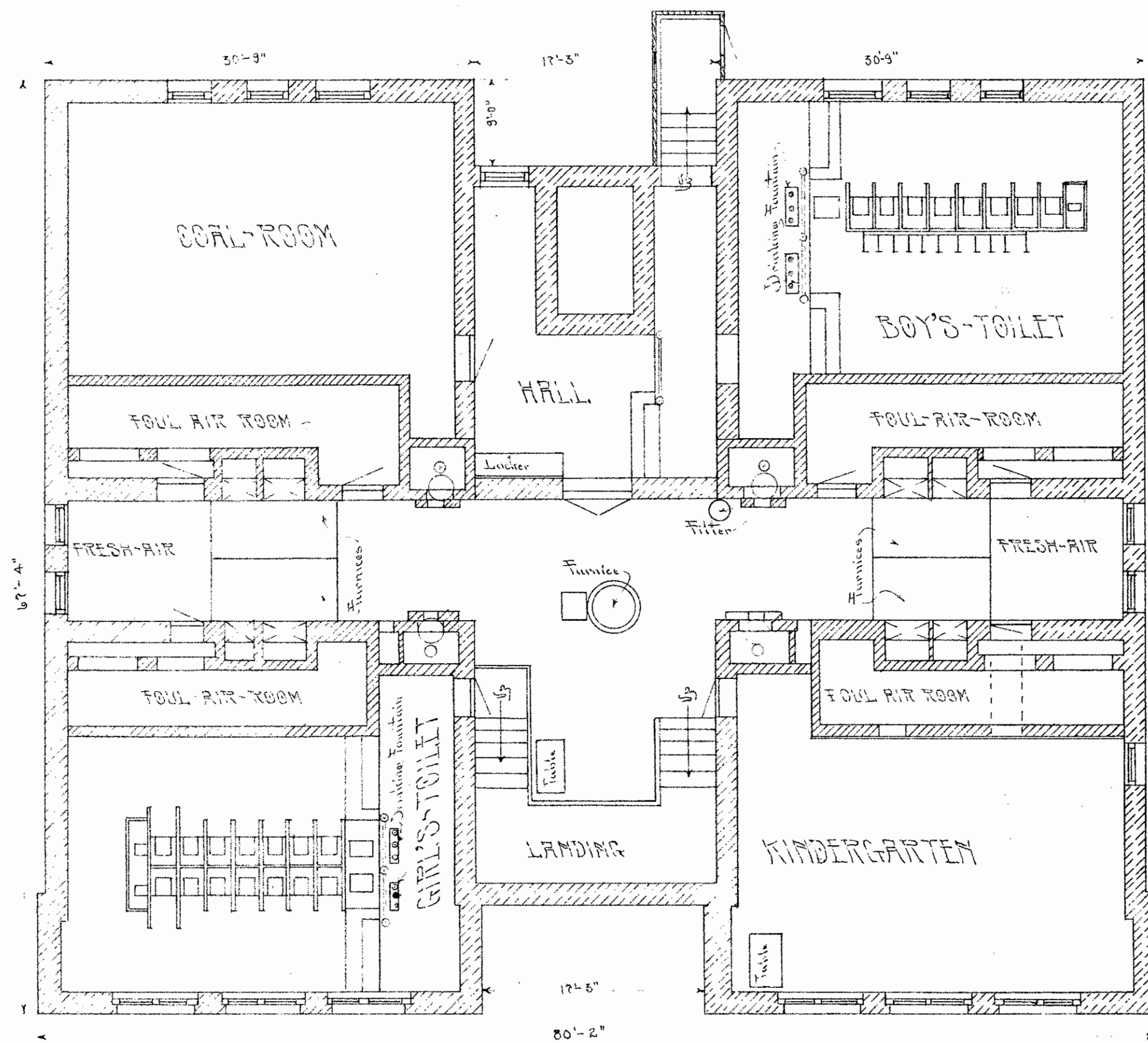
BASEMENT-FLOOR-PLAN
