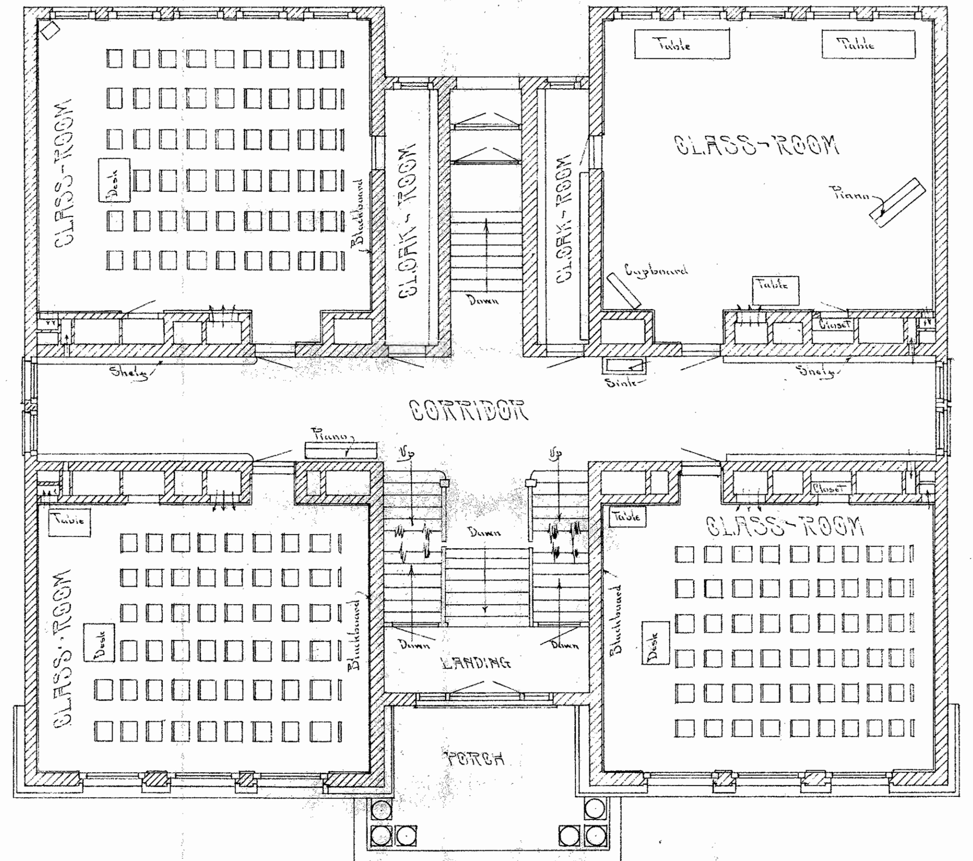
FIRST-FLOOR-PLAN
