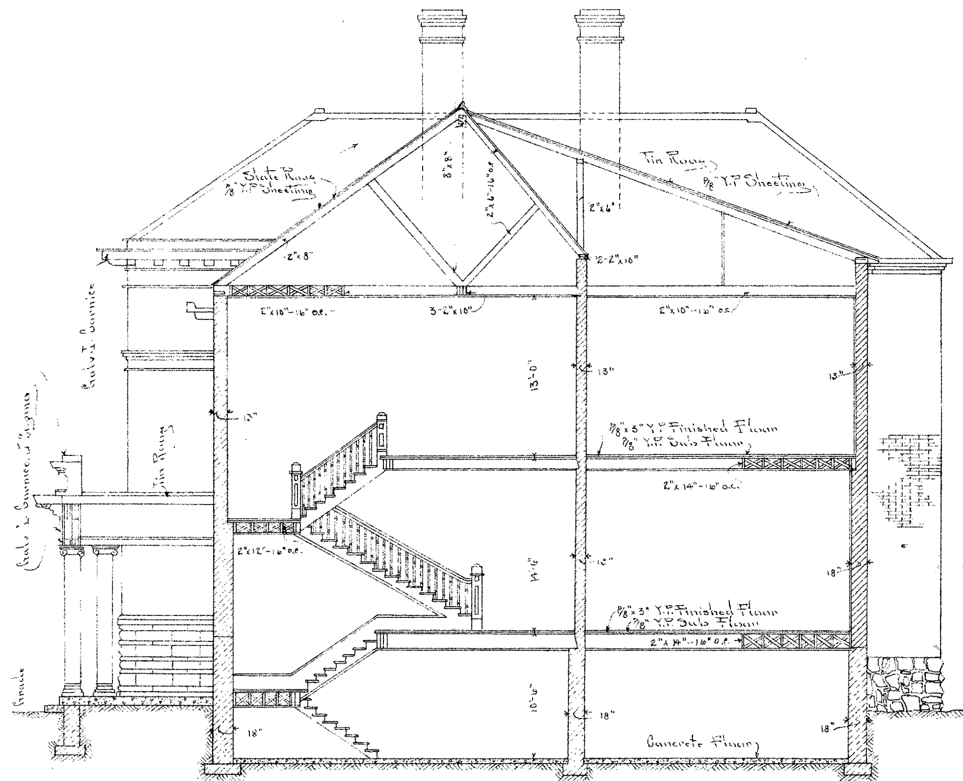
CROSS - SECTION
