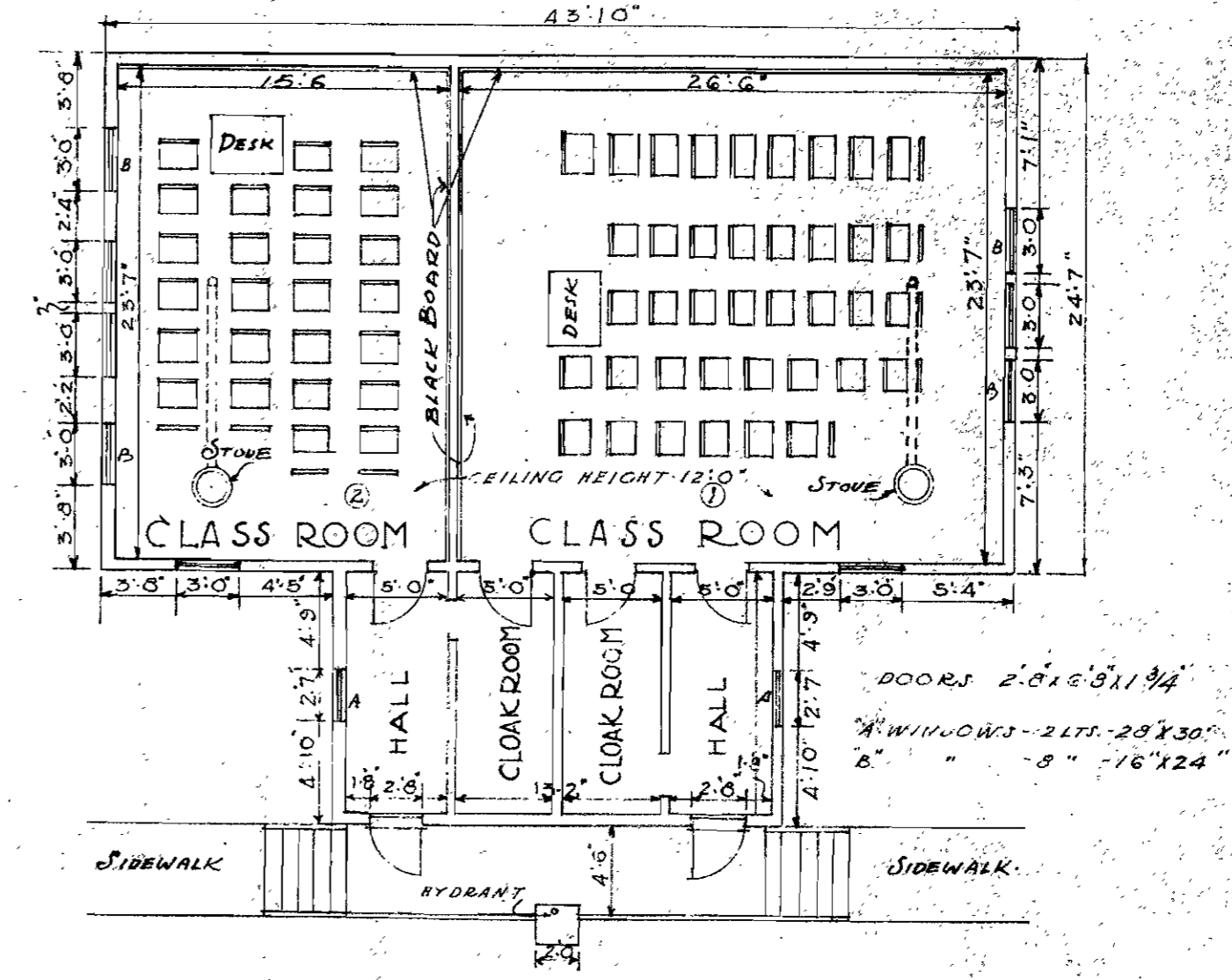
FLOOR PLAN
