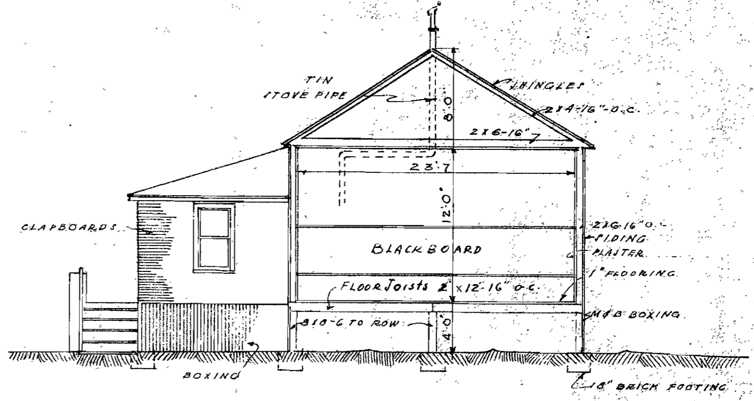
SECTION
