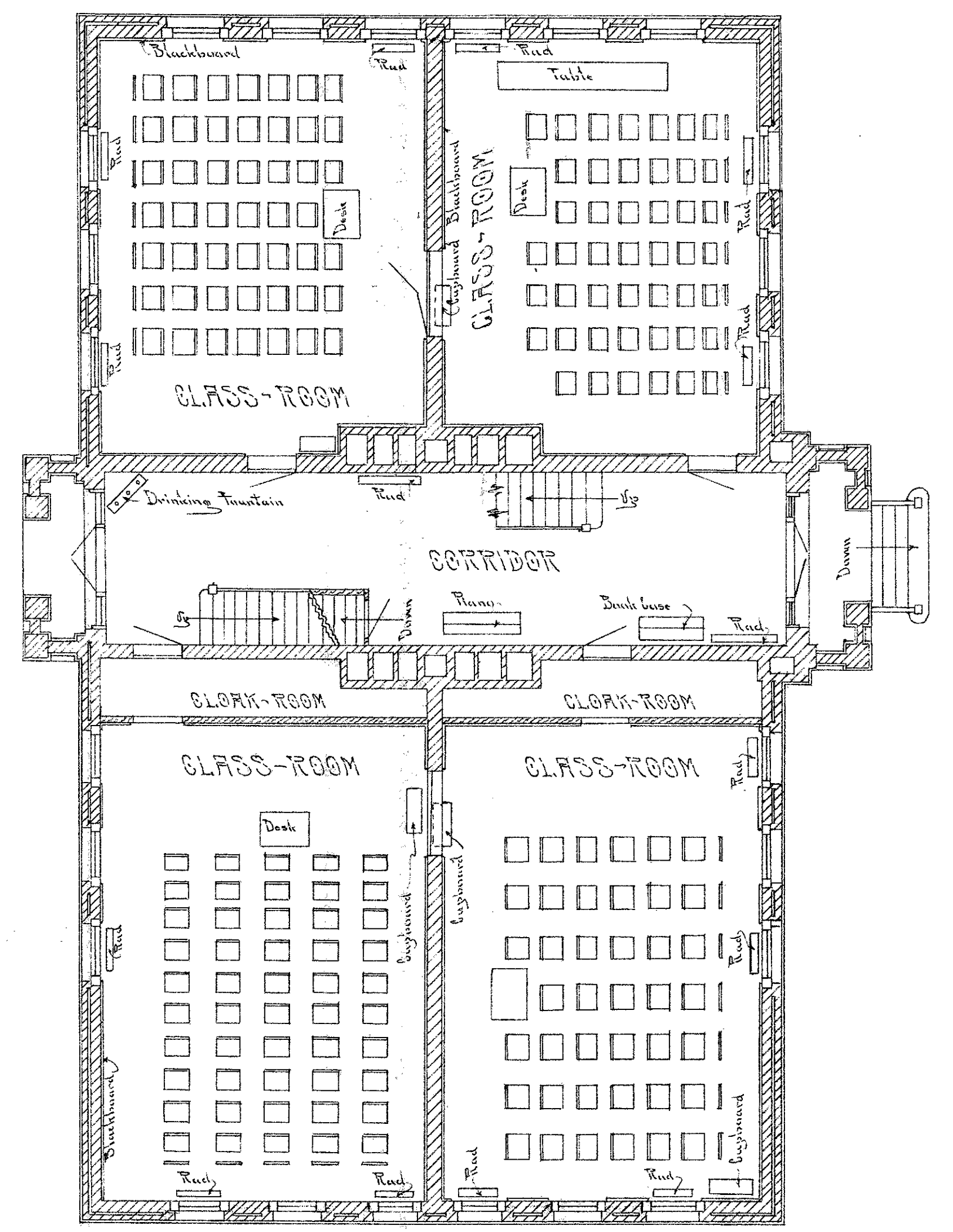
FIRST-FLOOR-PLAN
