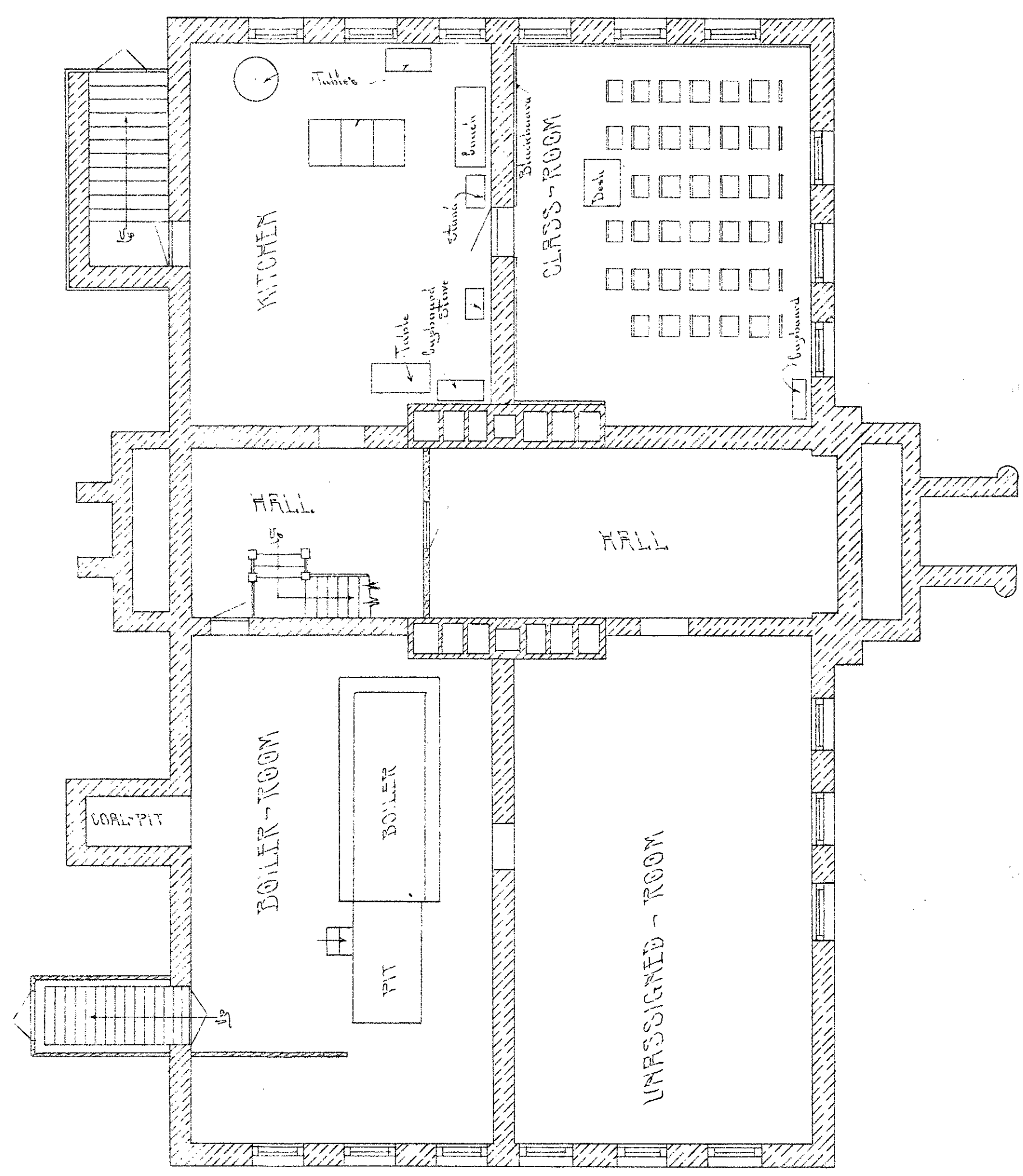
BASMENT-FLOOR-PLAN
