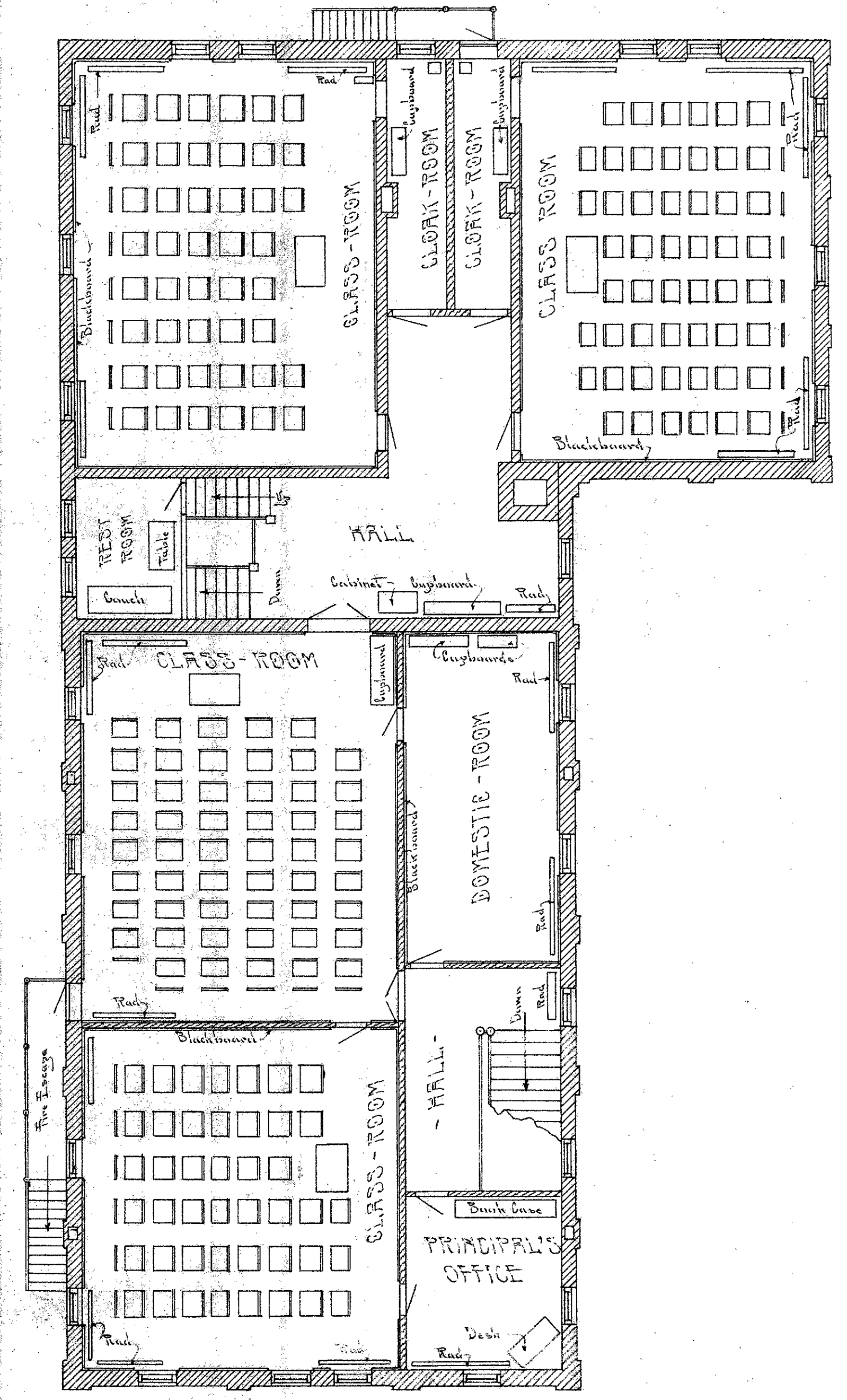
SECOND-FLOOR-PLAN
