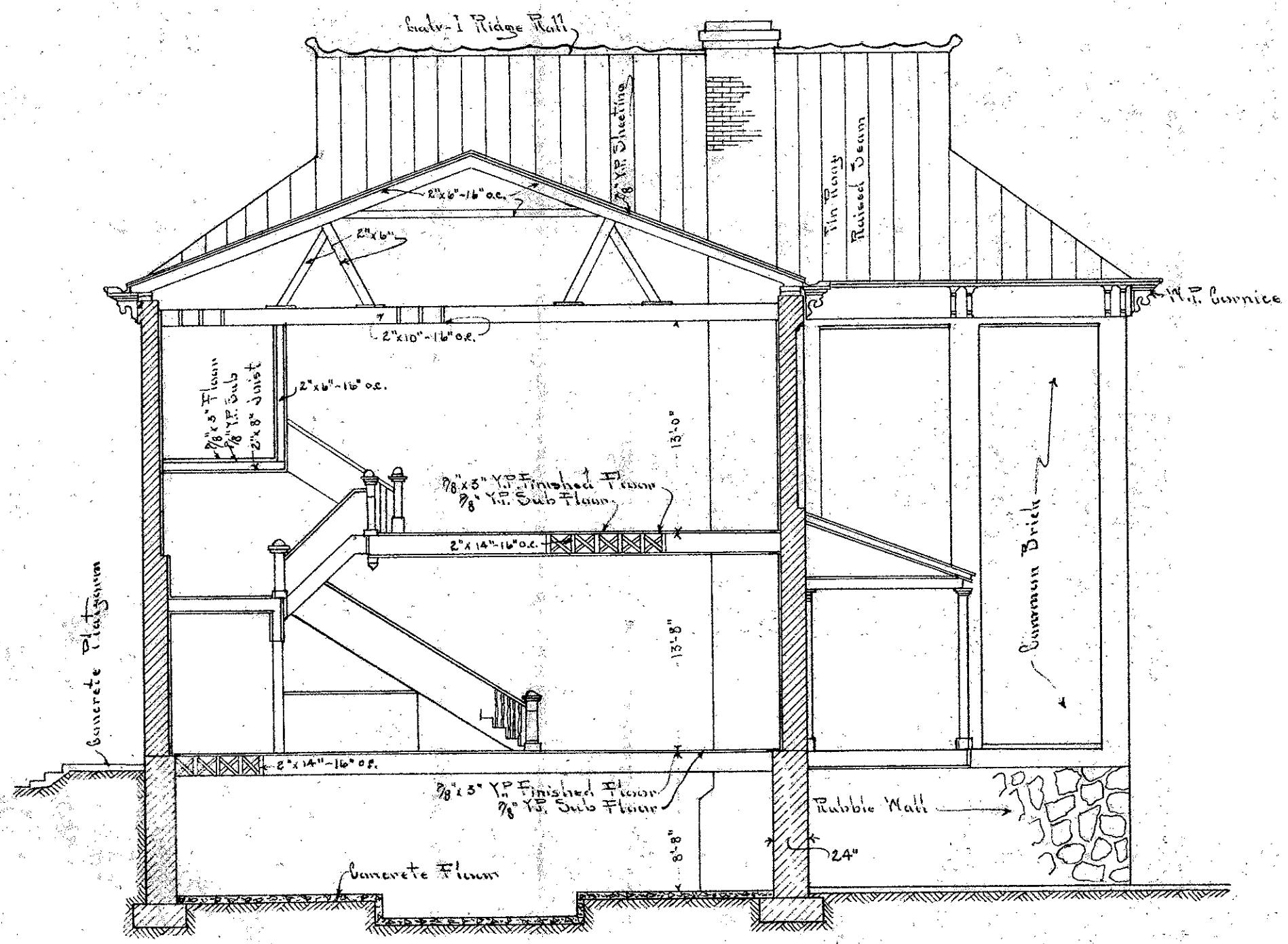
CROSS-SECTION
