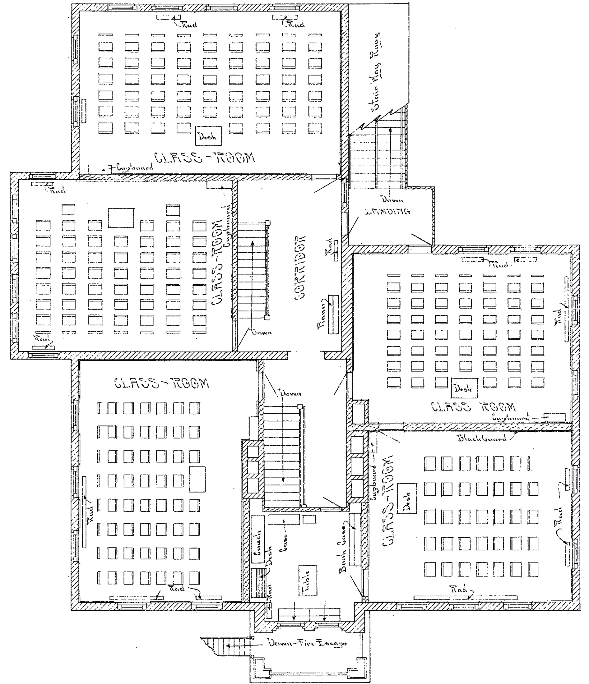
SECOND-FLOOR-PLAN
