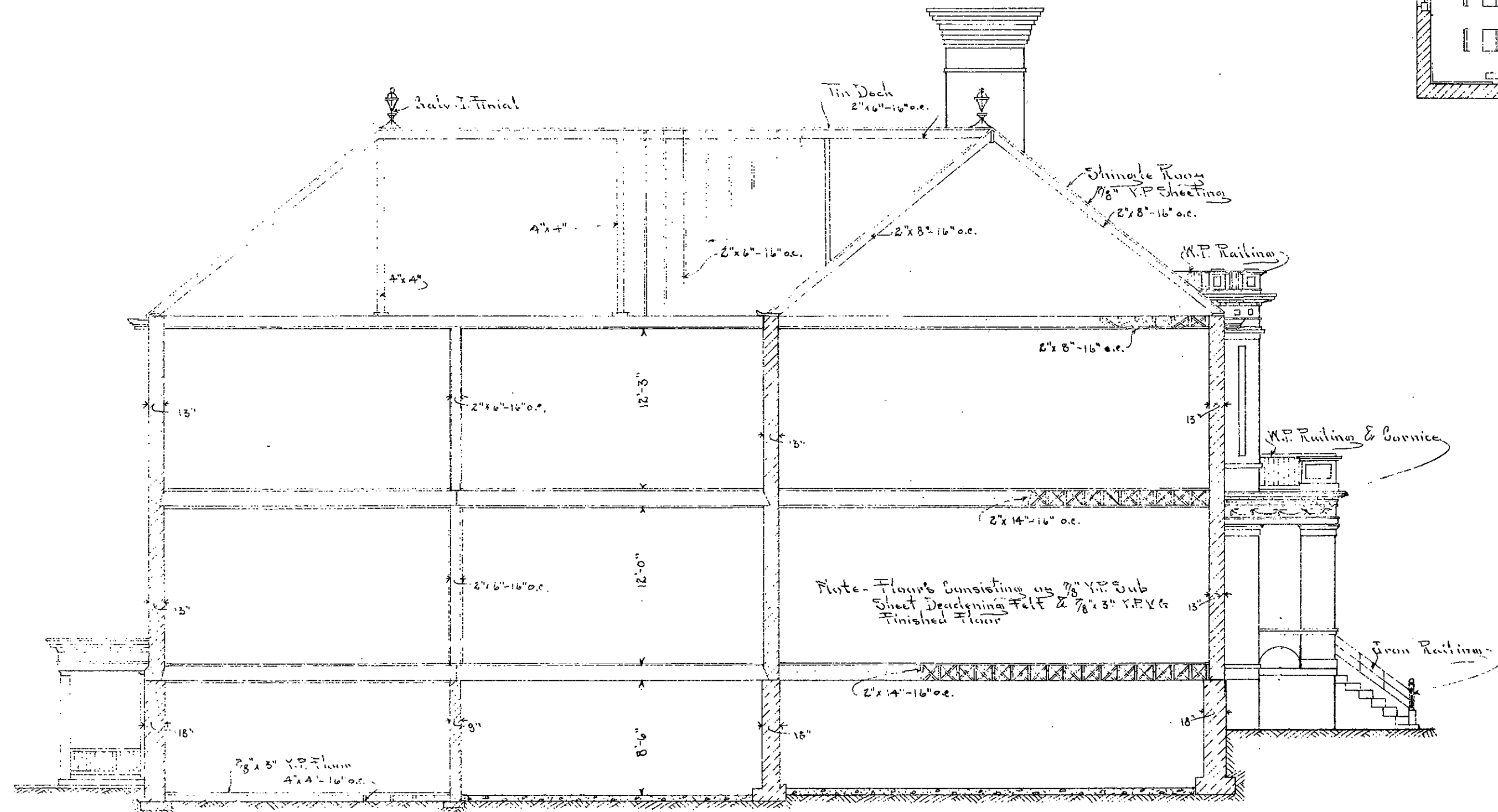
CROSS-SECTION-LOOKING-NORTH
