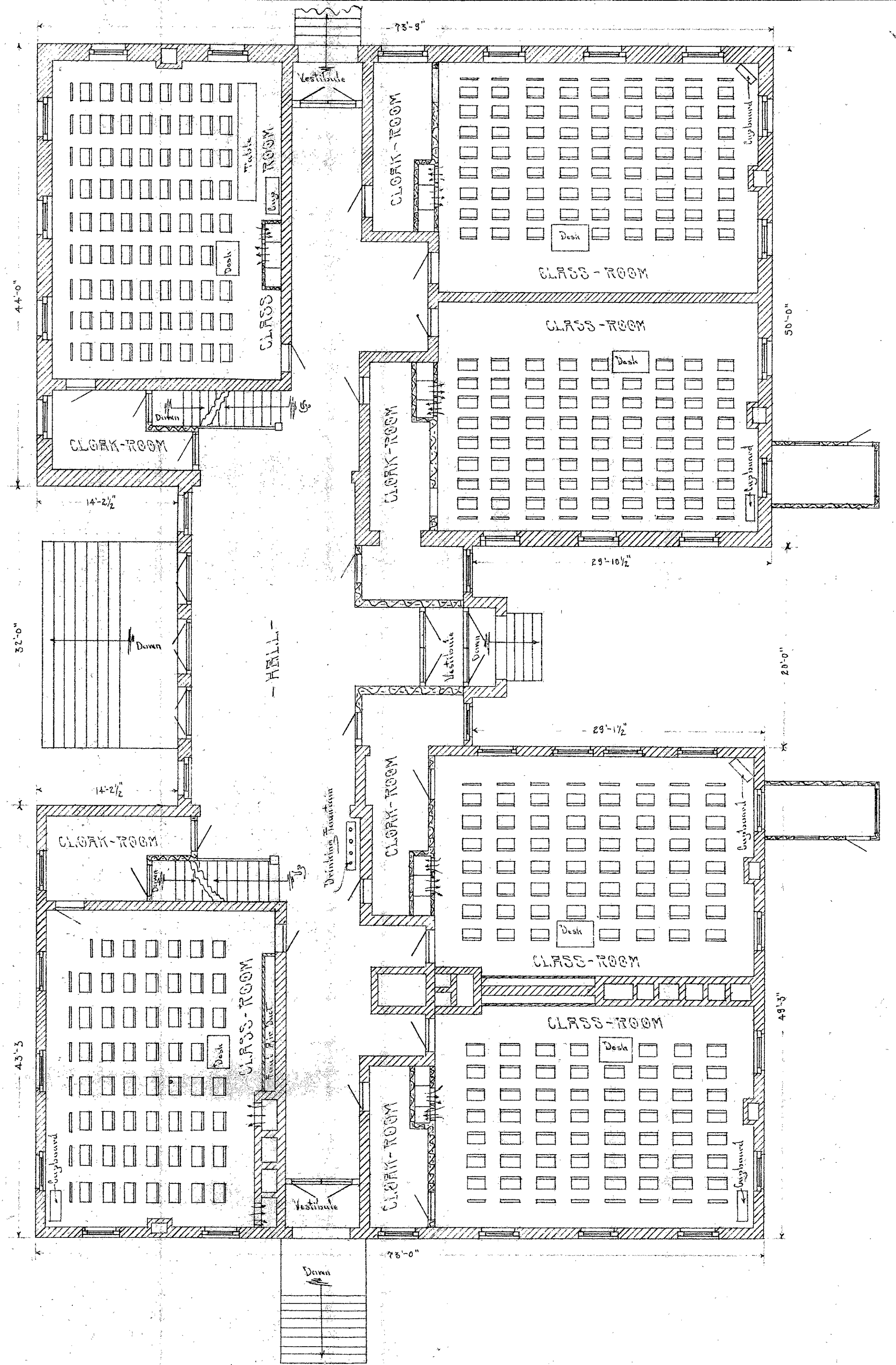
FIRST-FLOOR-PLAN
