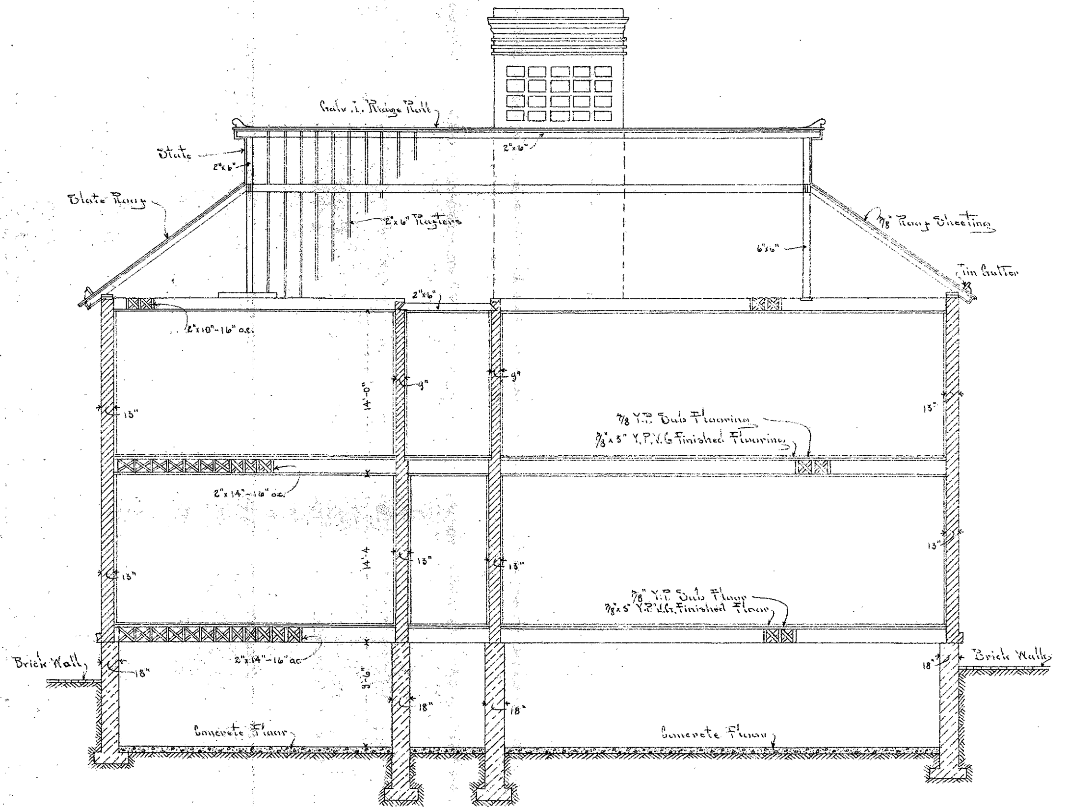
CROSS - SECTION - LOOKING - WEST
