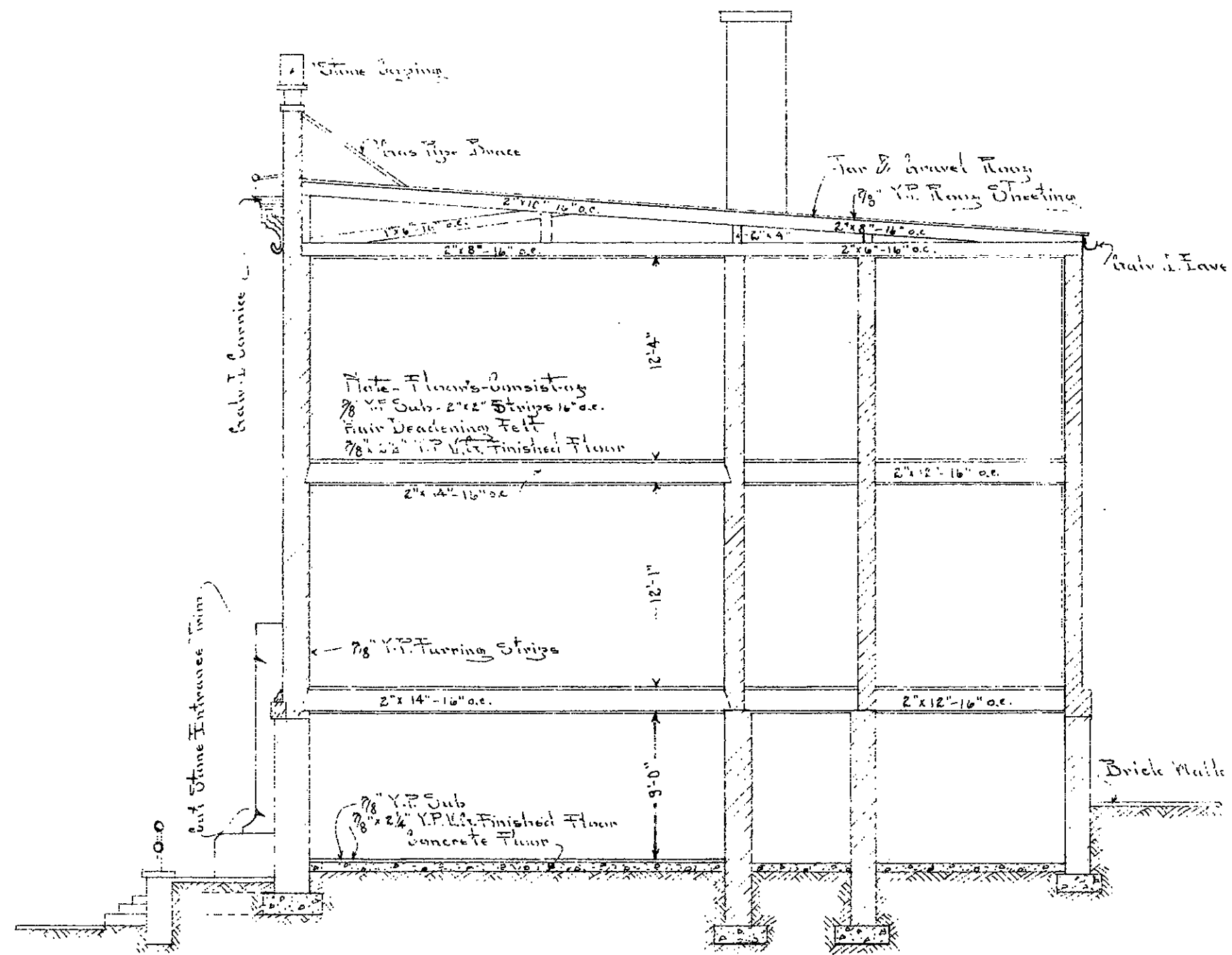
CROSS-SECTION
