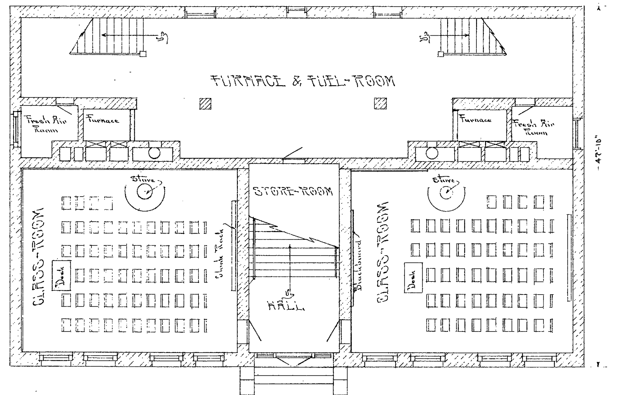
BASMENT-FLOOR-PLAN
