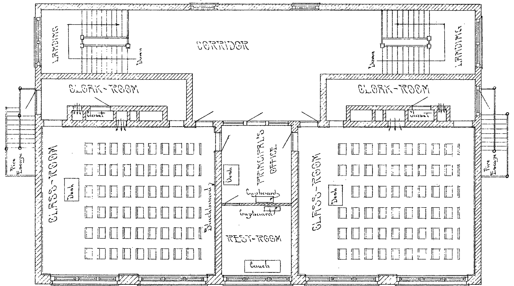
SECOND-FLOOR-PLAN
