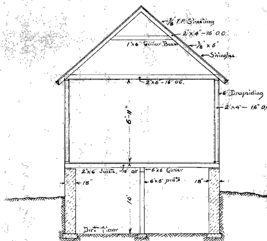
CROSS-SECTION
