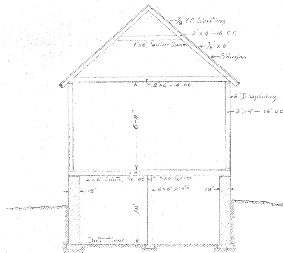
CROSS-SECTION
