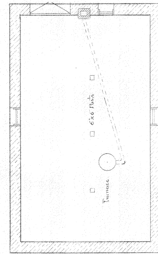
BASEMENT-FLOOR-PLAN
