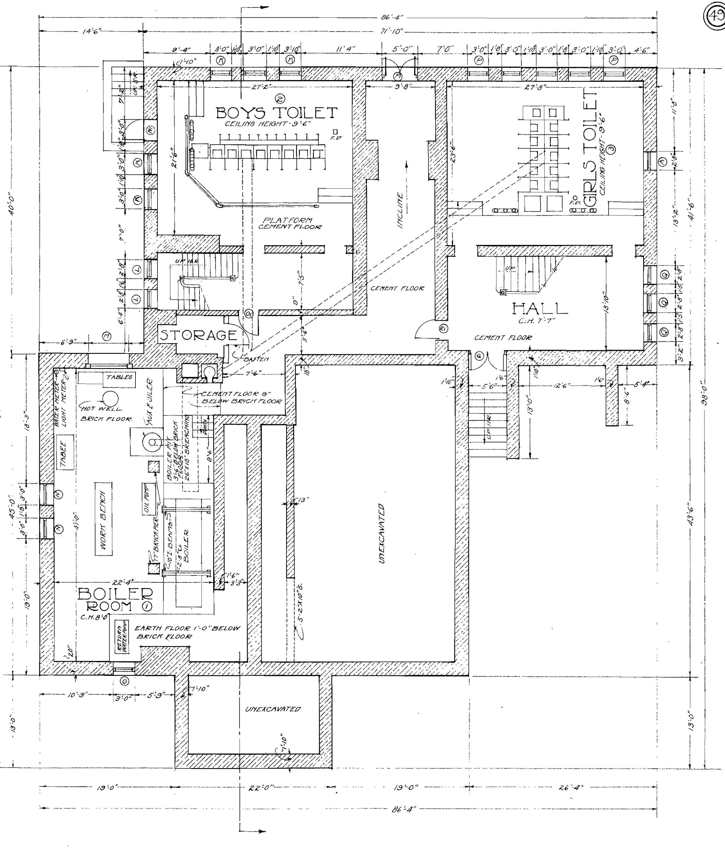
BASEMENT PLAN
