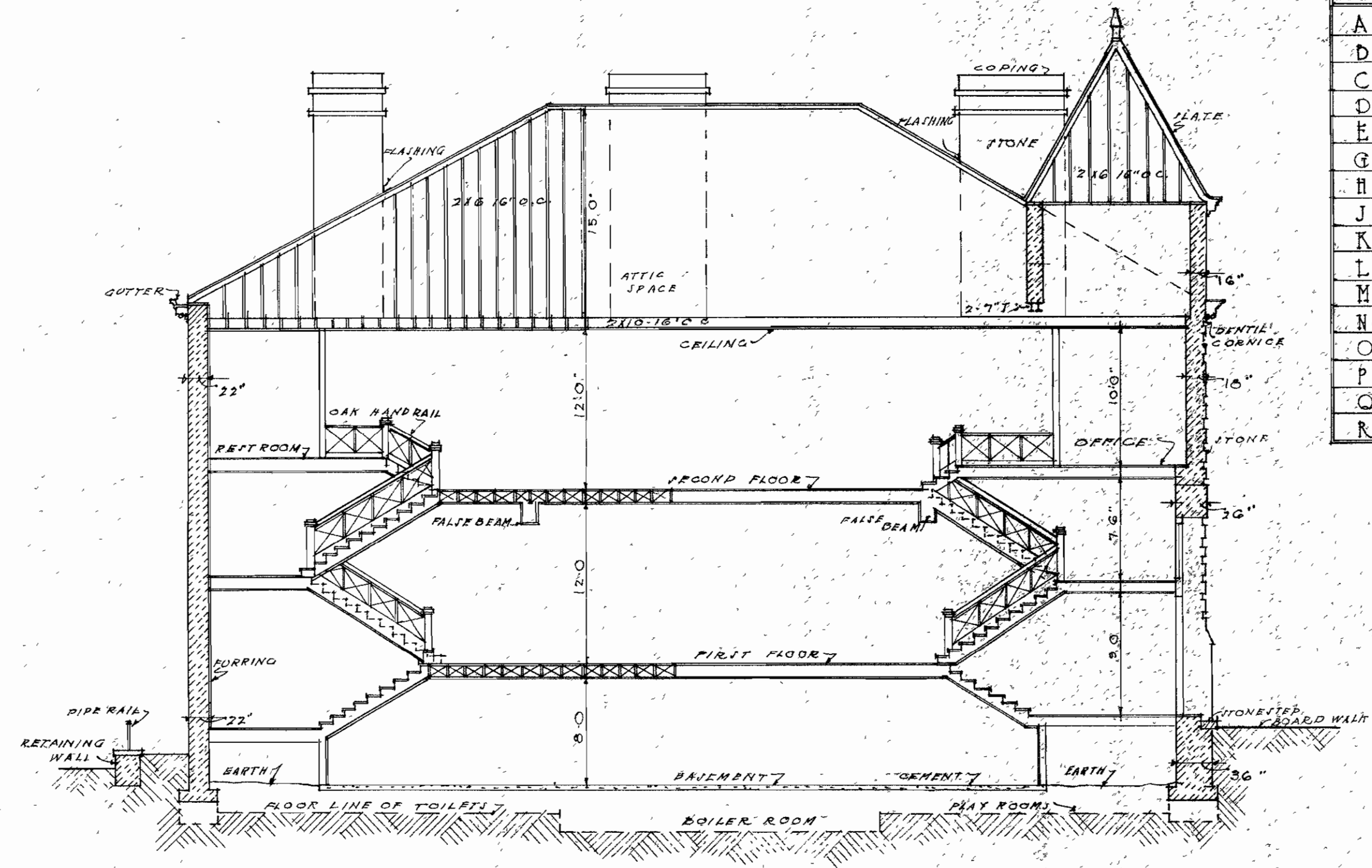
CROSS - SECTION
