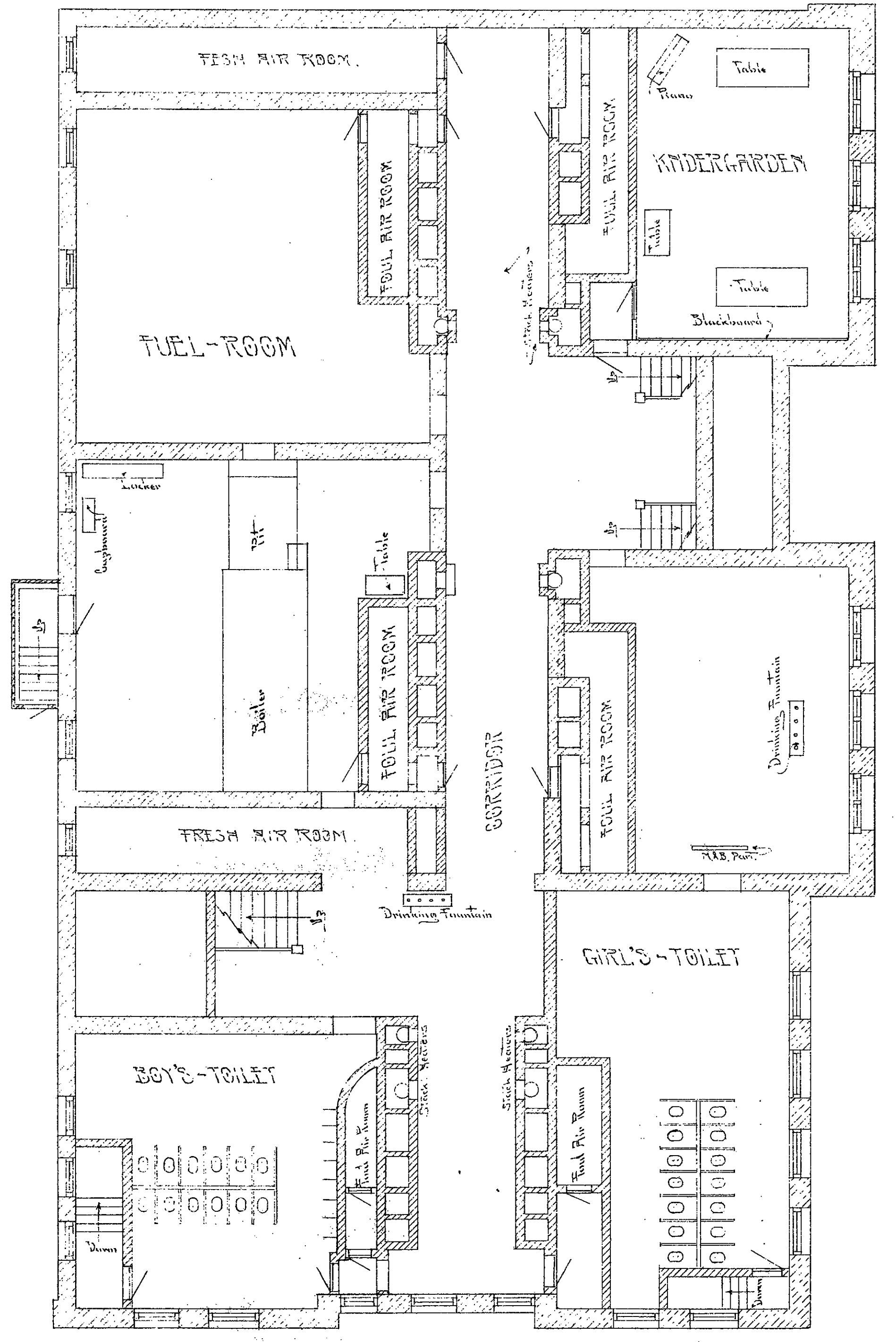
BASEMENT-FLOOR-PLAN
