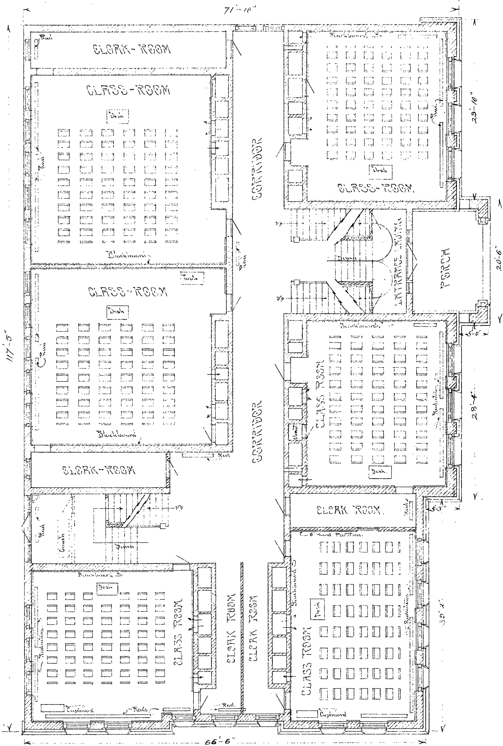
FIRST-FLOOR-PLAN
