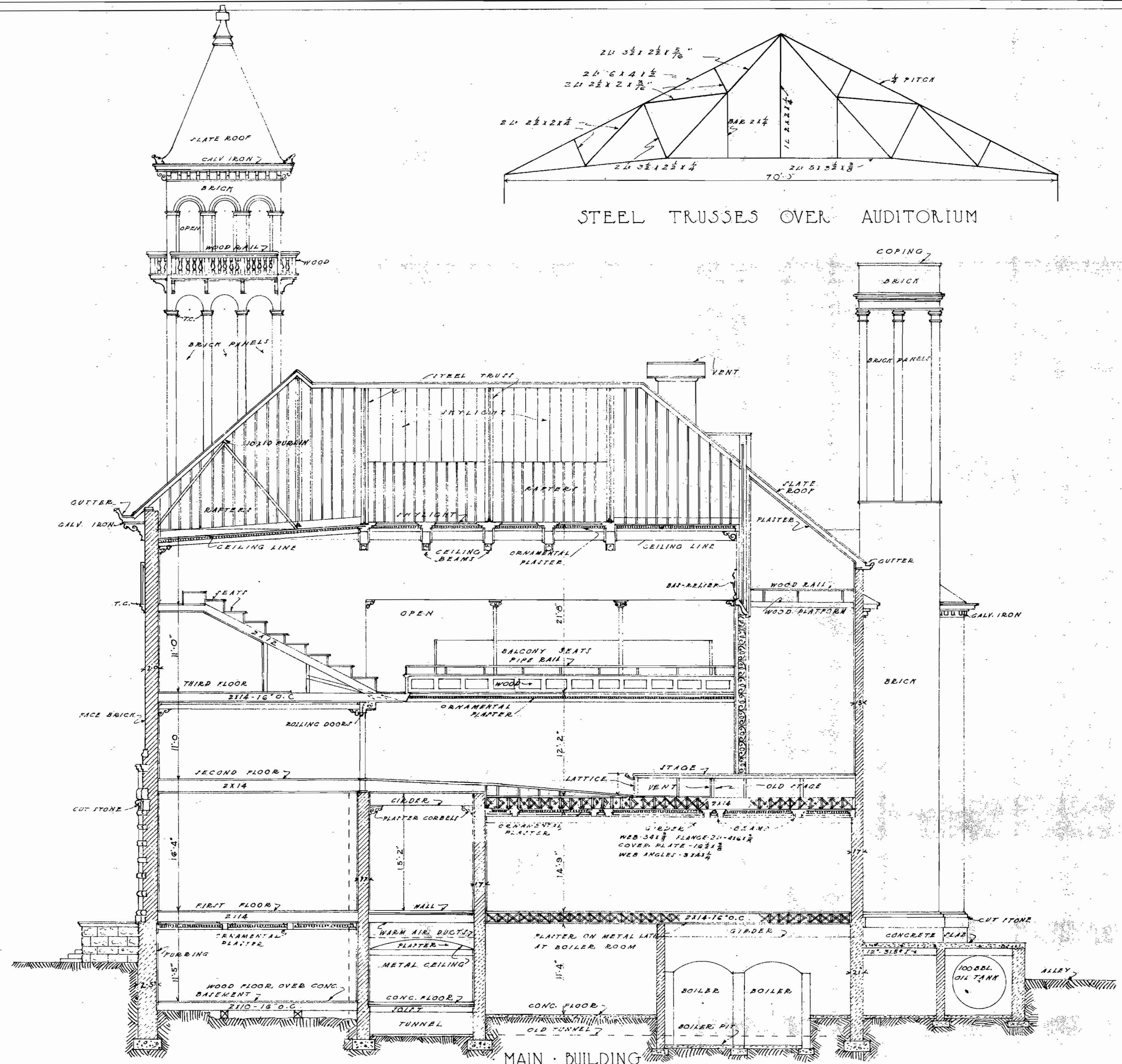
MAIN BUILDING CROSS SECTION SCALE 1/4" = 1'-0"
