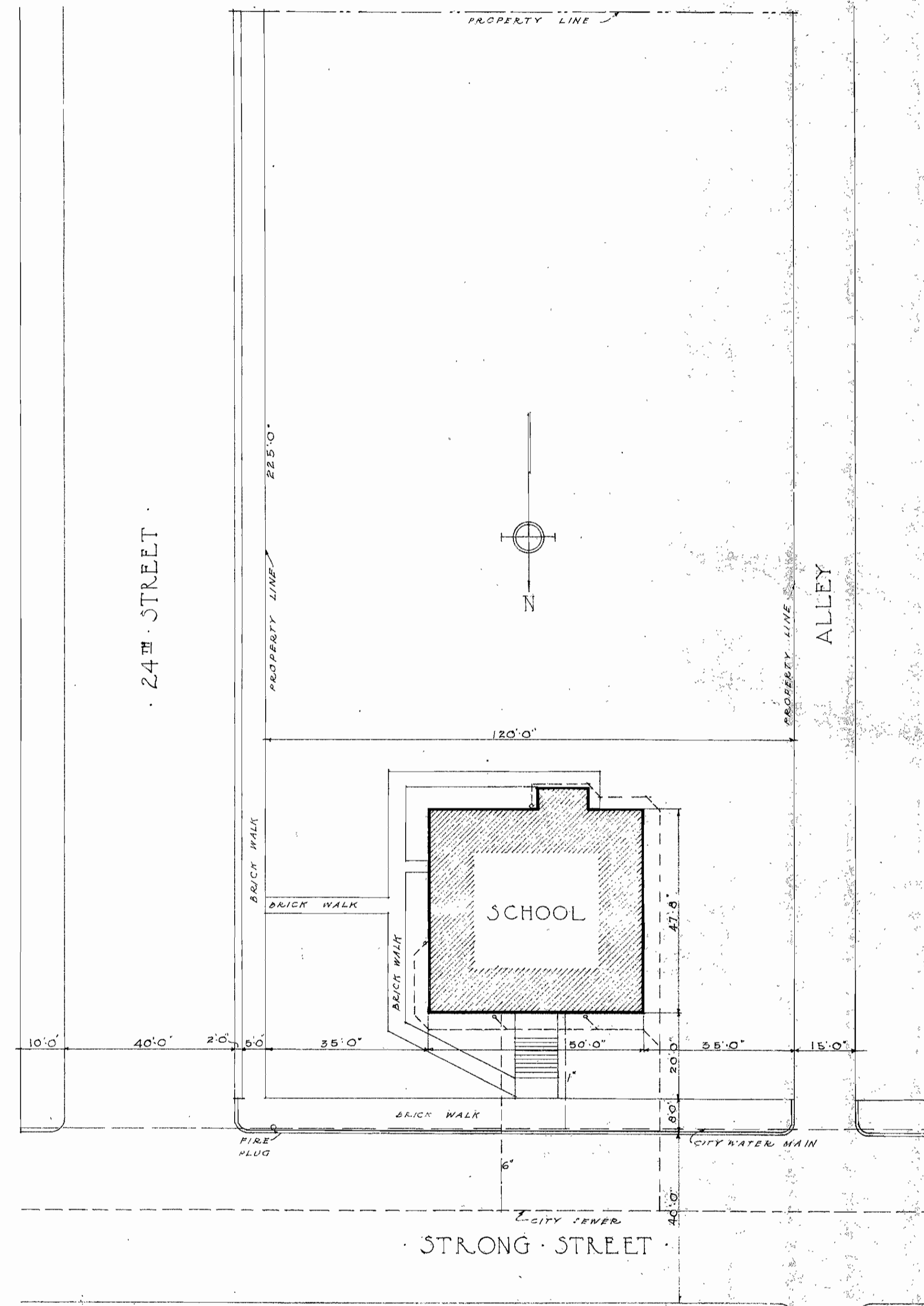
PLOT PLAN SCALE 0 5 10 15 20 30
