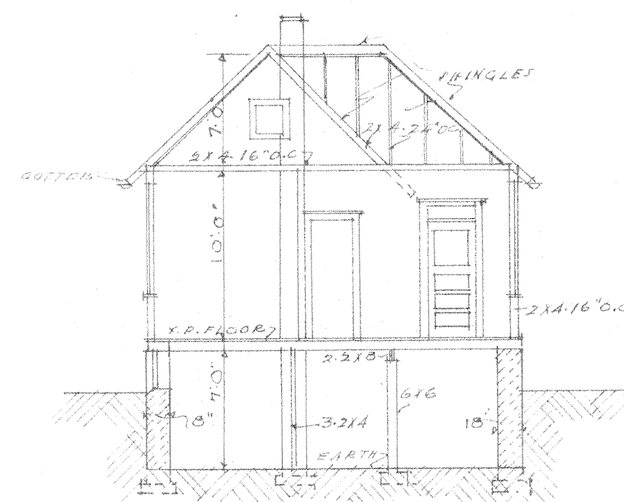
SECTION
