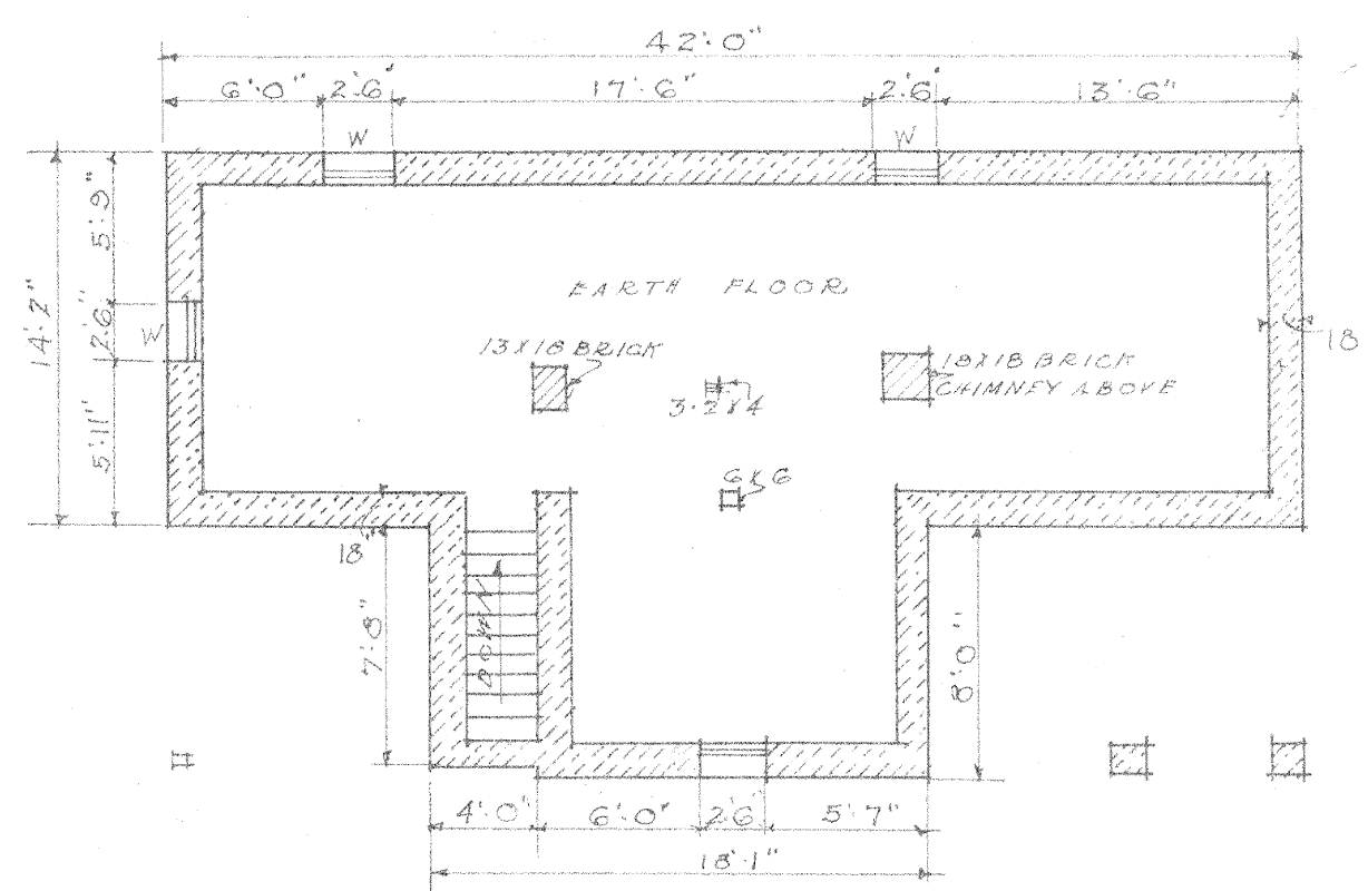
BASEMENT PLAN
