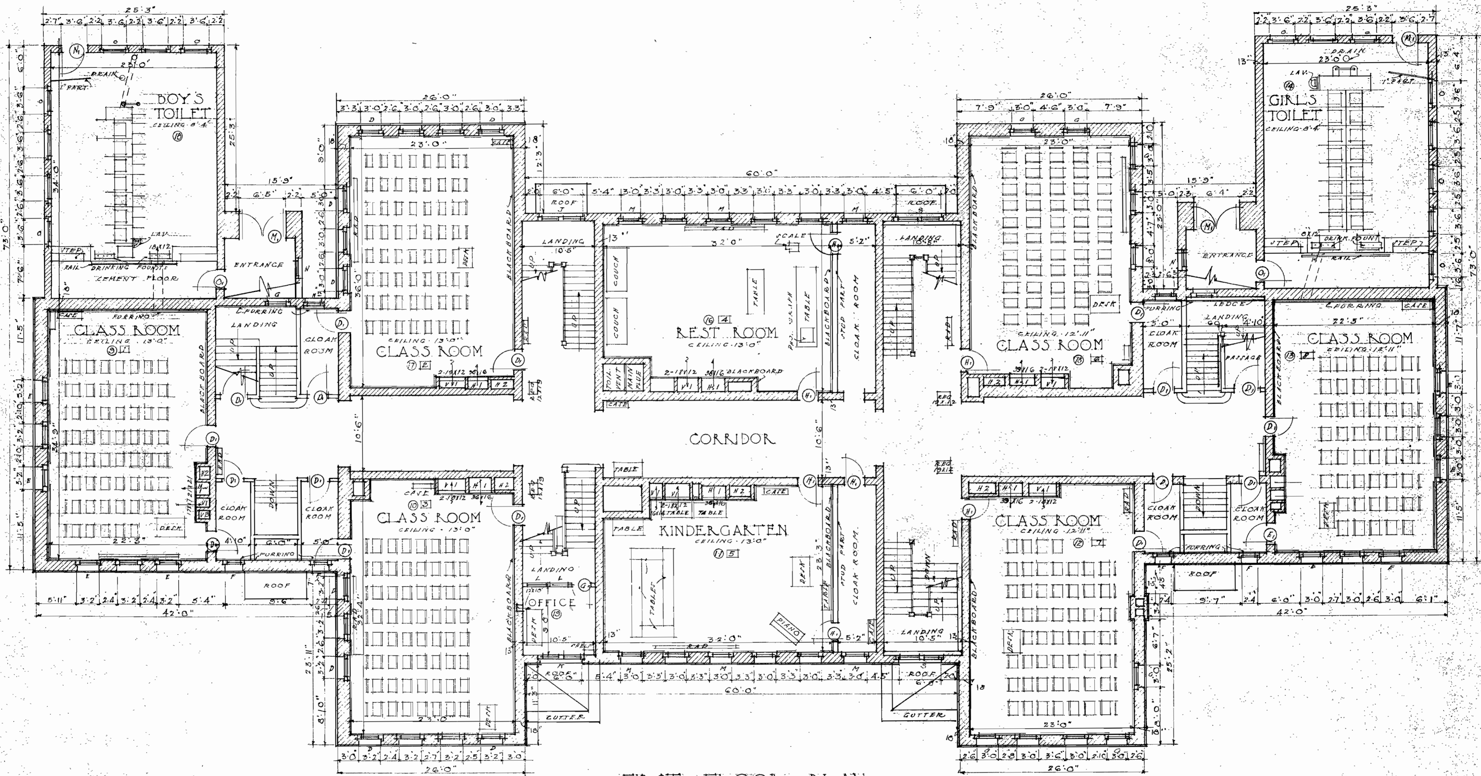
FIRST FLOOR PLAN SCALE 0 2 4 6 8 12
