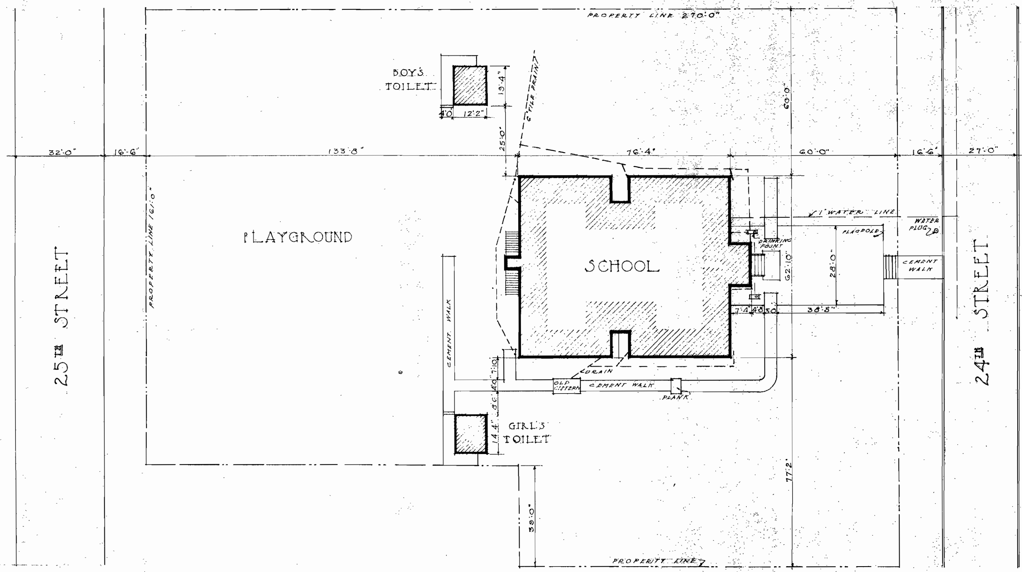
PLOT PLAN SCALE 0 5 10 15 20 25
