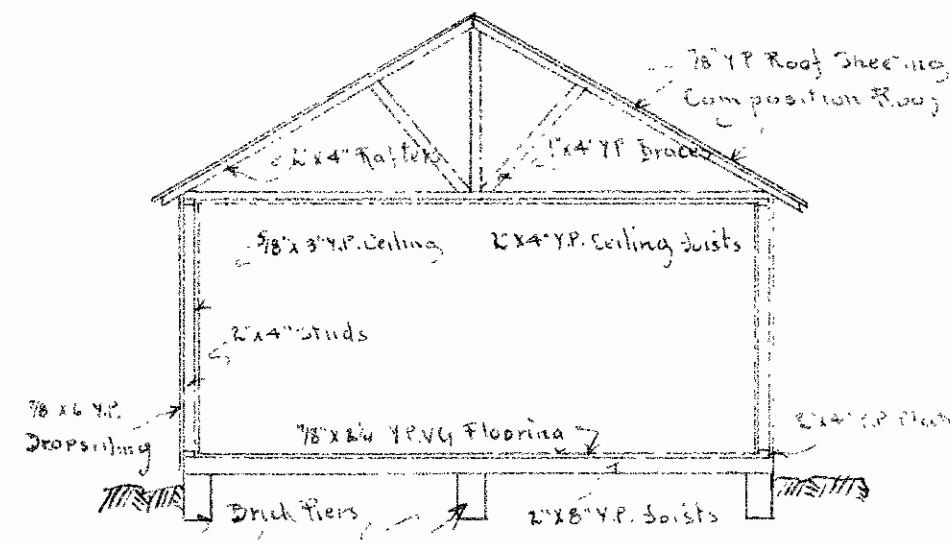
CROSS SECTION
