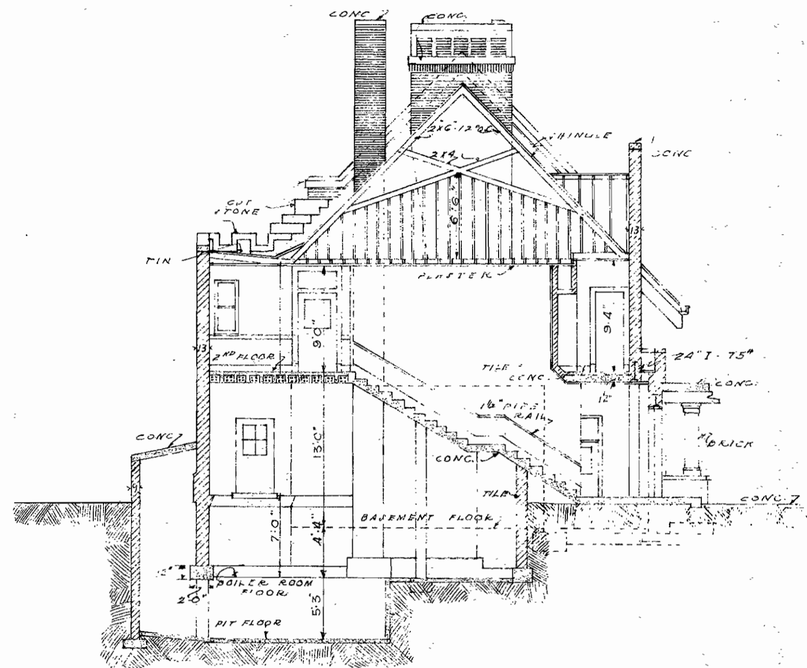
CROSS SECTION
