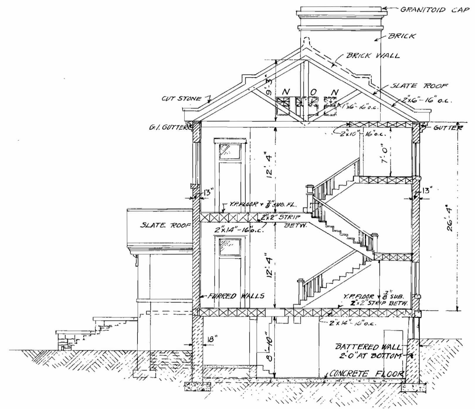
CROSS SECTION SCALE 0 2 4 6 8 12
