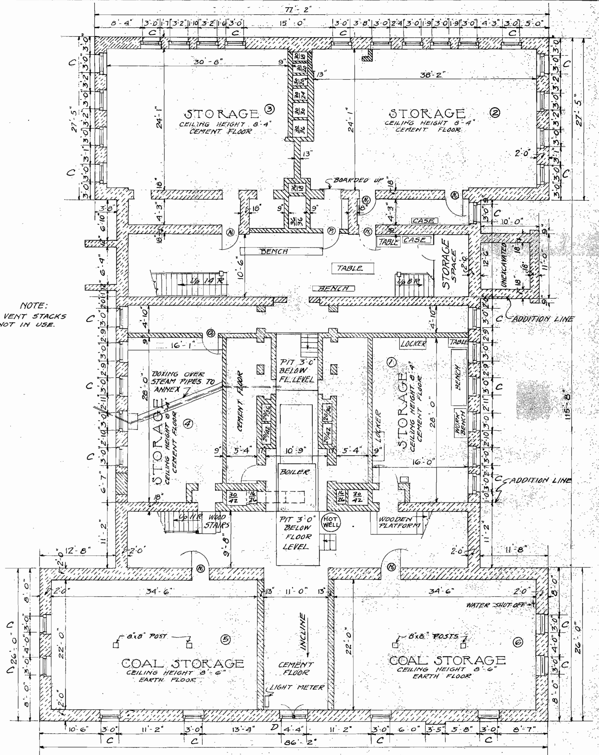
BASEMENT PLAN
