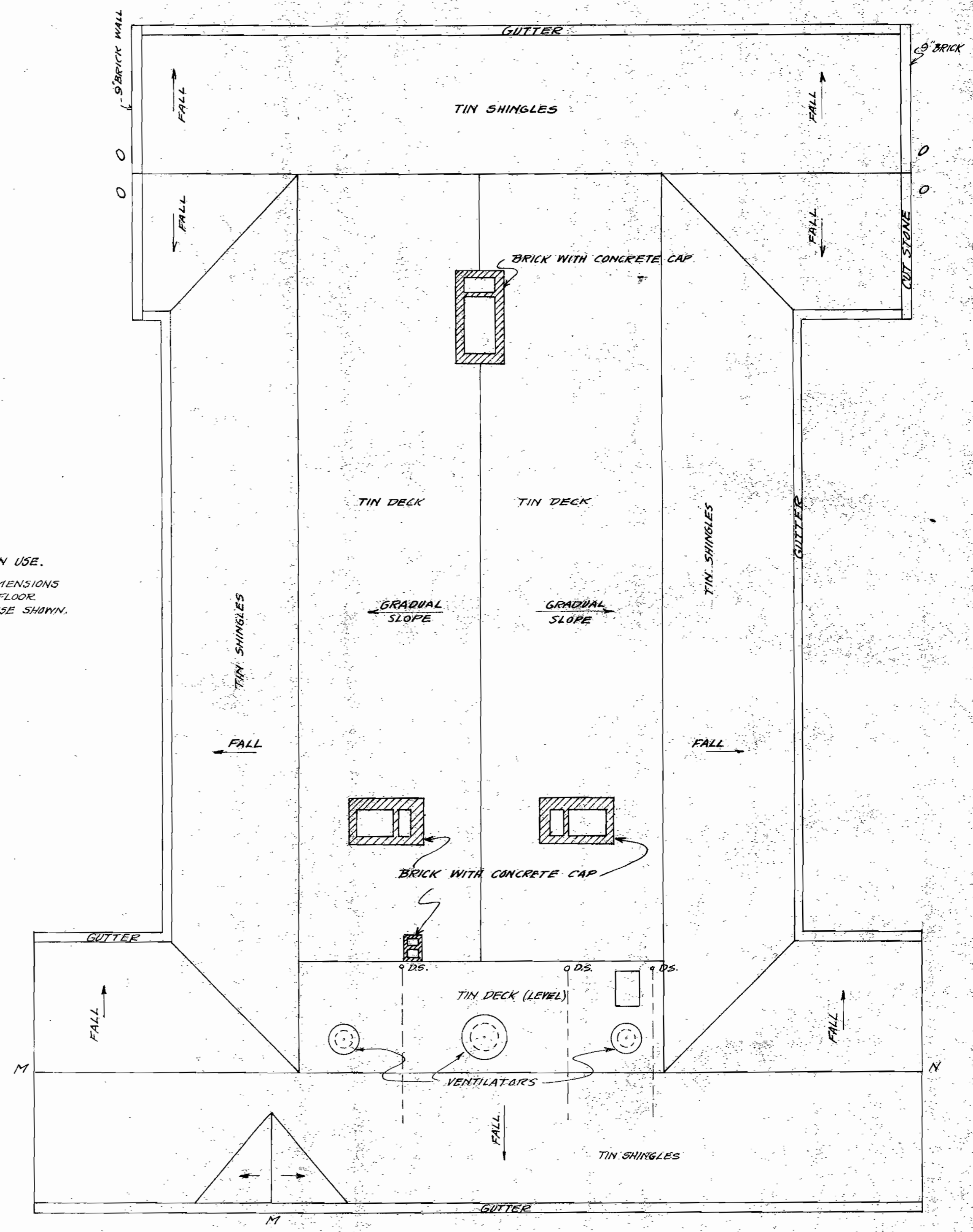
ROOF PLAN
