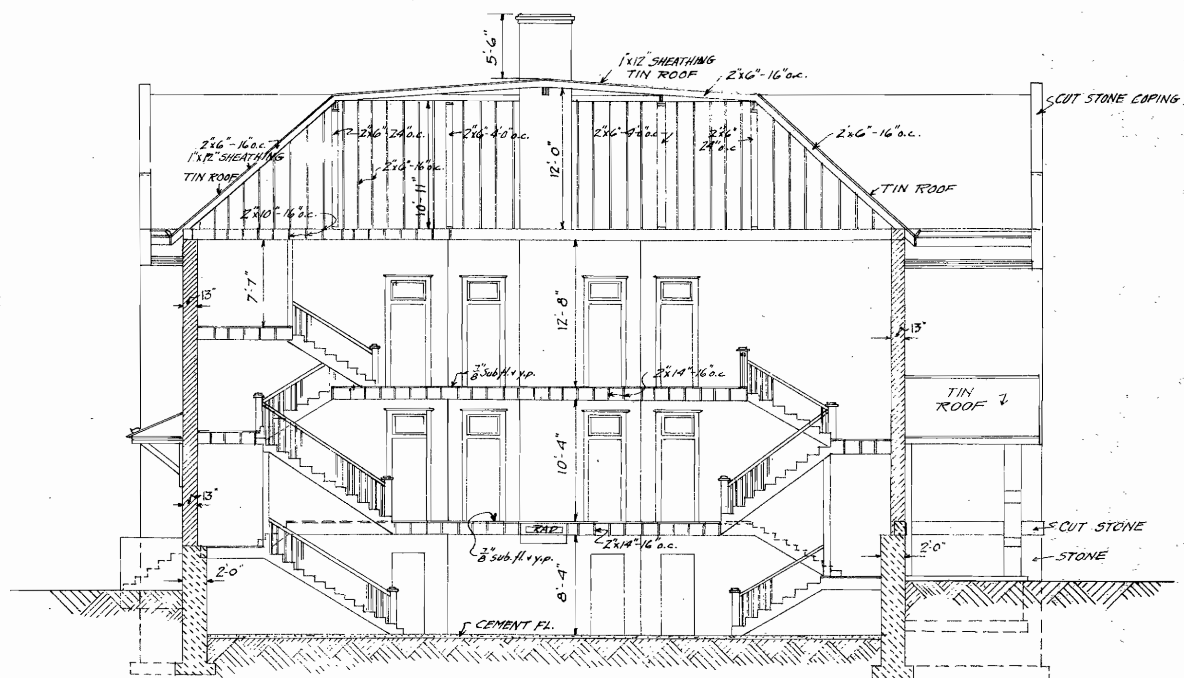
CROSS SECTION SCALE 0 2 4 6 8 12
