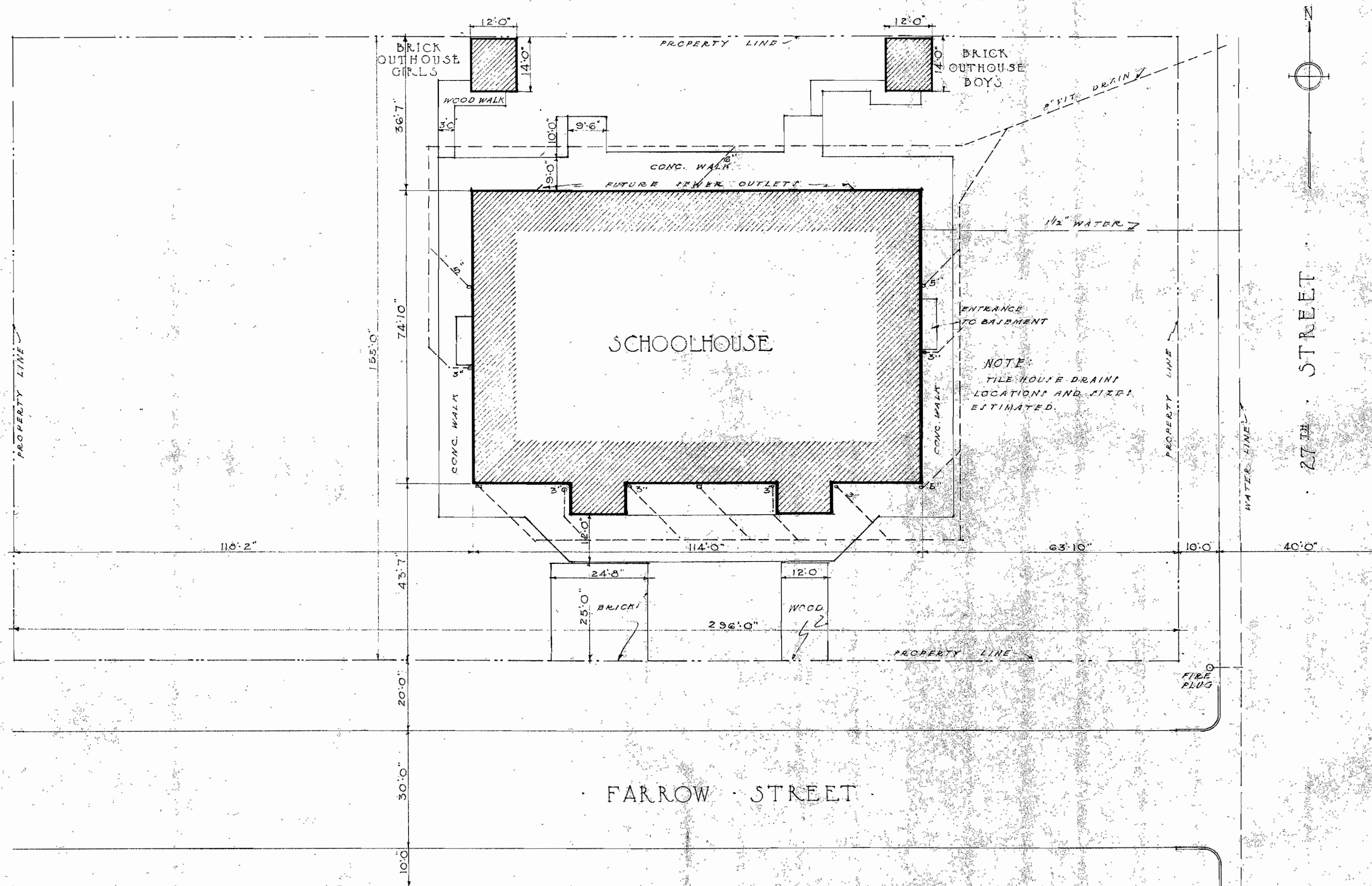
PLOT PLAN SCALE 0 5 10 15 20 30
