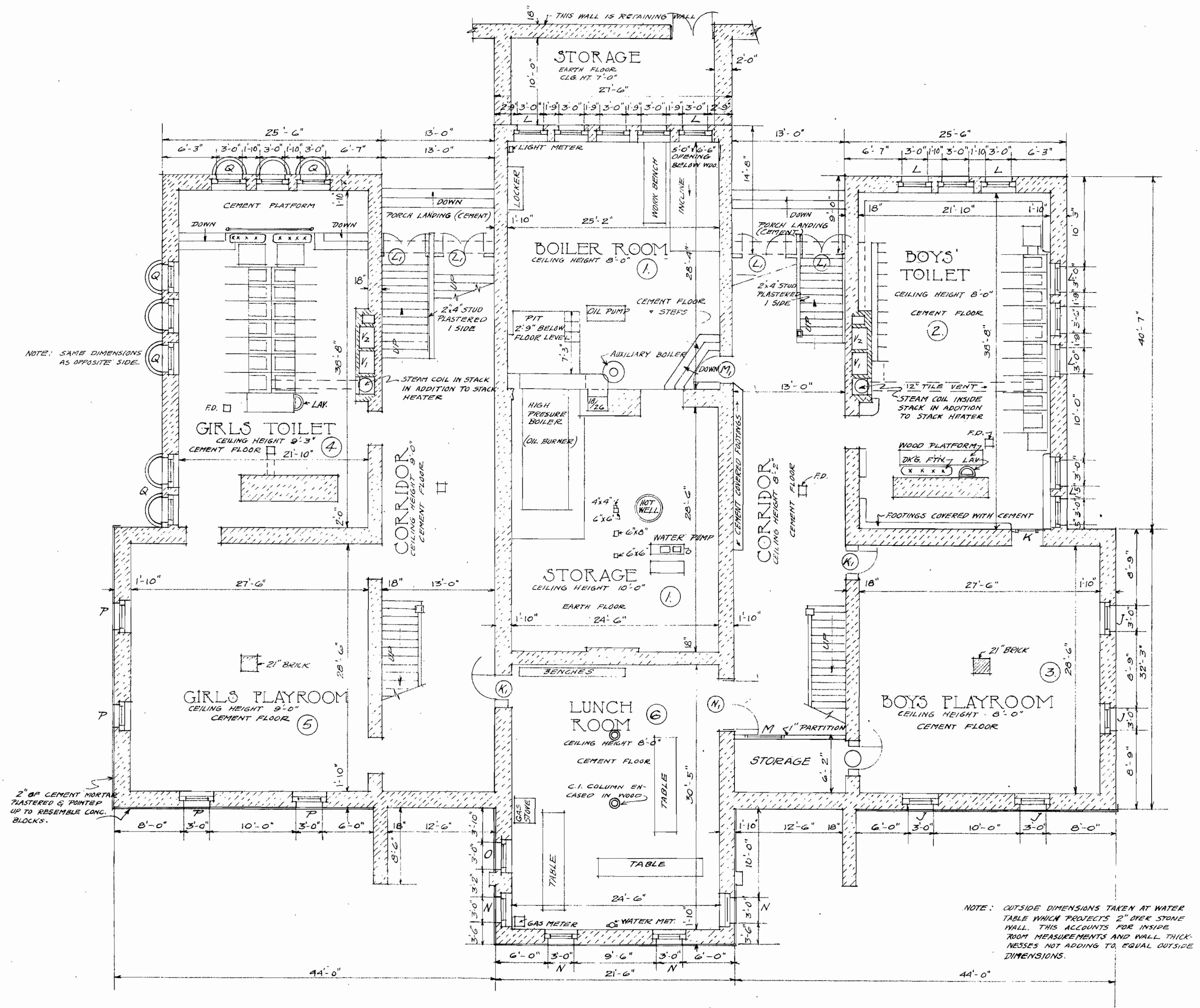
BASEMENT PLAN SCALE 0 2 4 6 8 12
