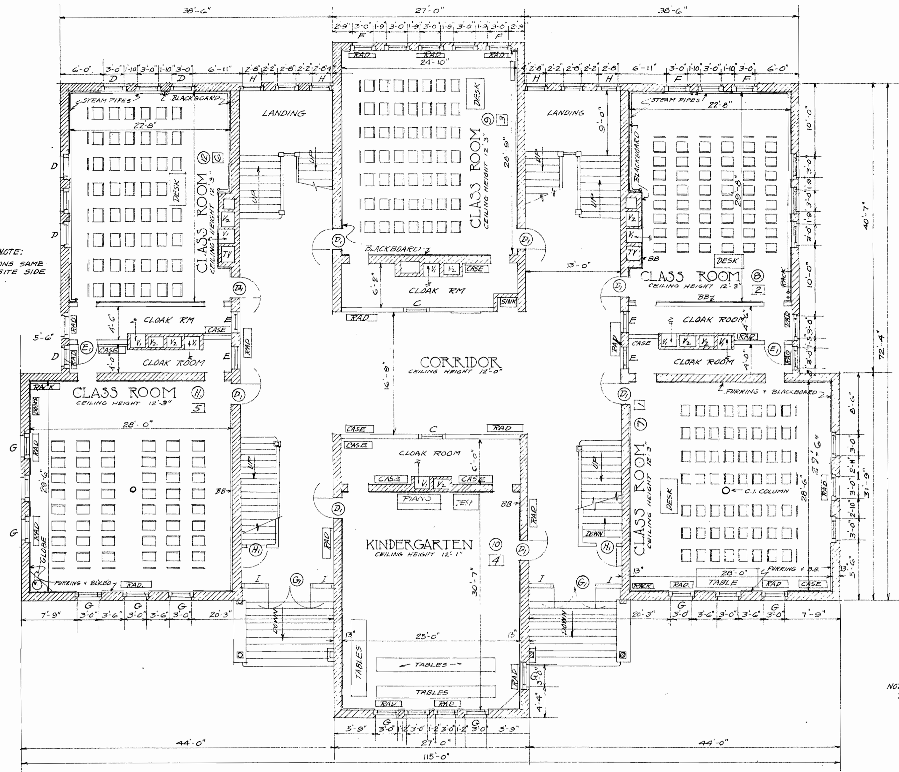
FIRST FLOOR PLAN SCALE 0 2 4 6 8 12
