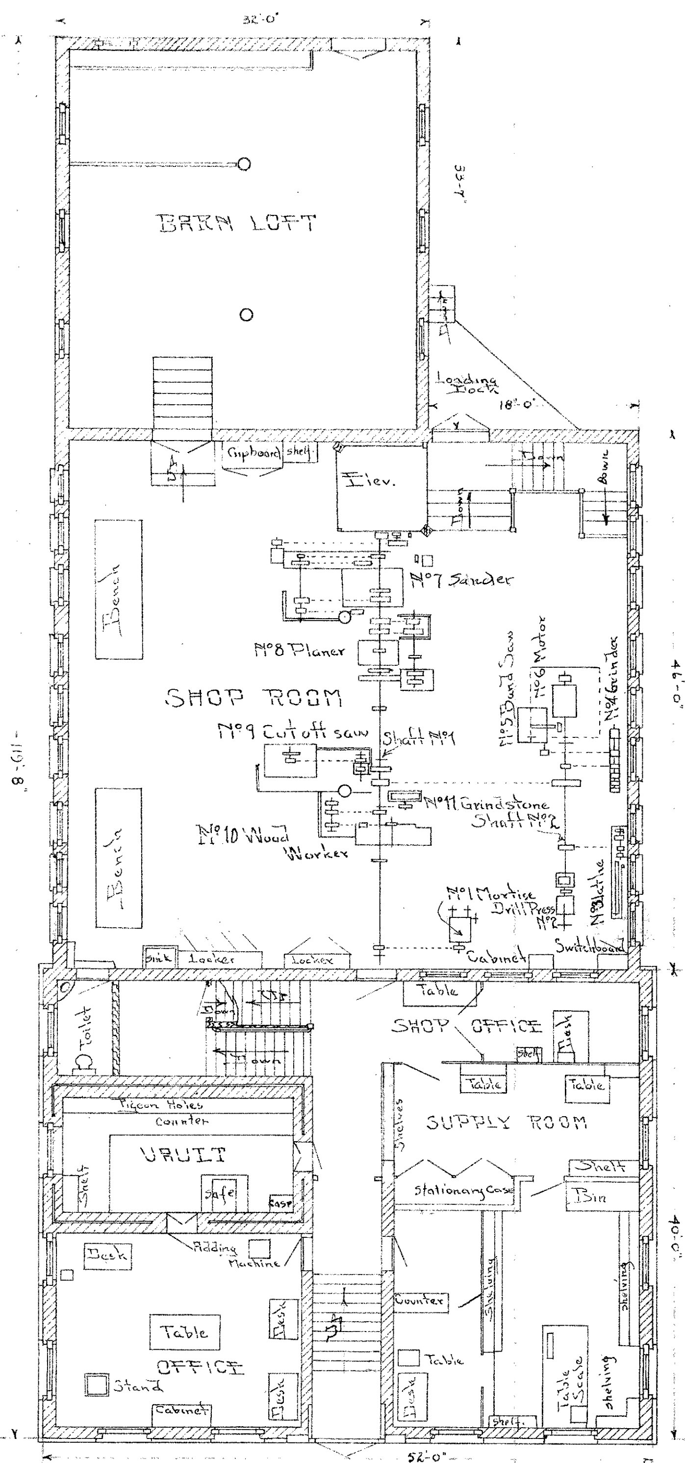
FIRST FLOOR
