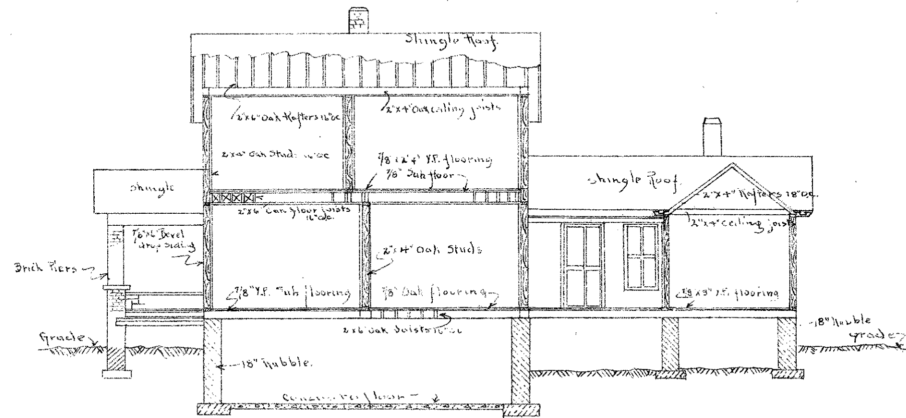
CROSS SECTION LOOKING NORTH SHOP RESIDENCE
