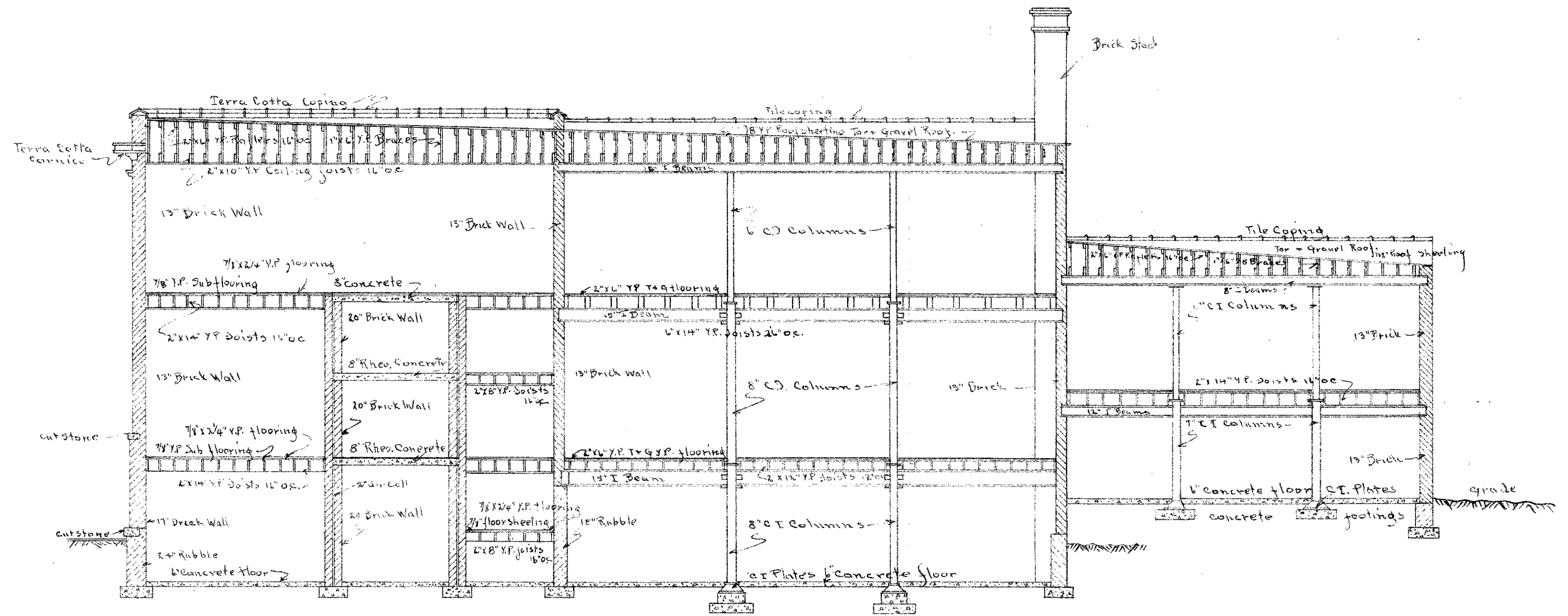
CROSS-SECTION OF SHOP LOOKING NORTH
