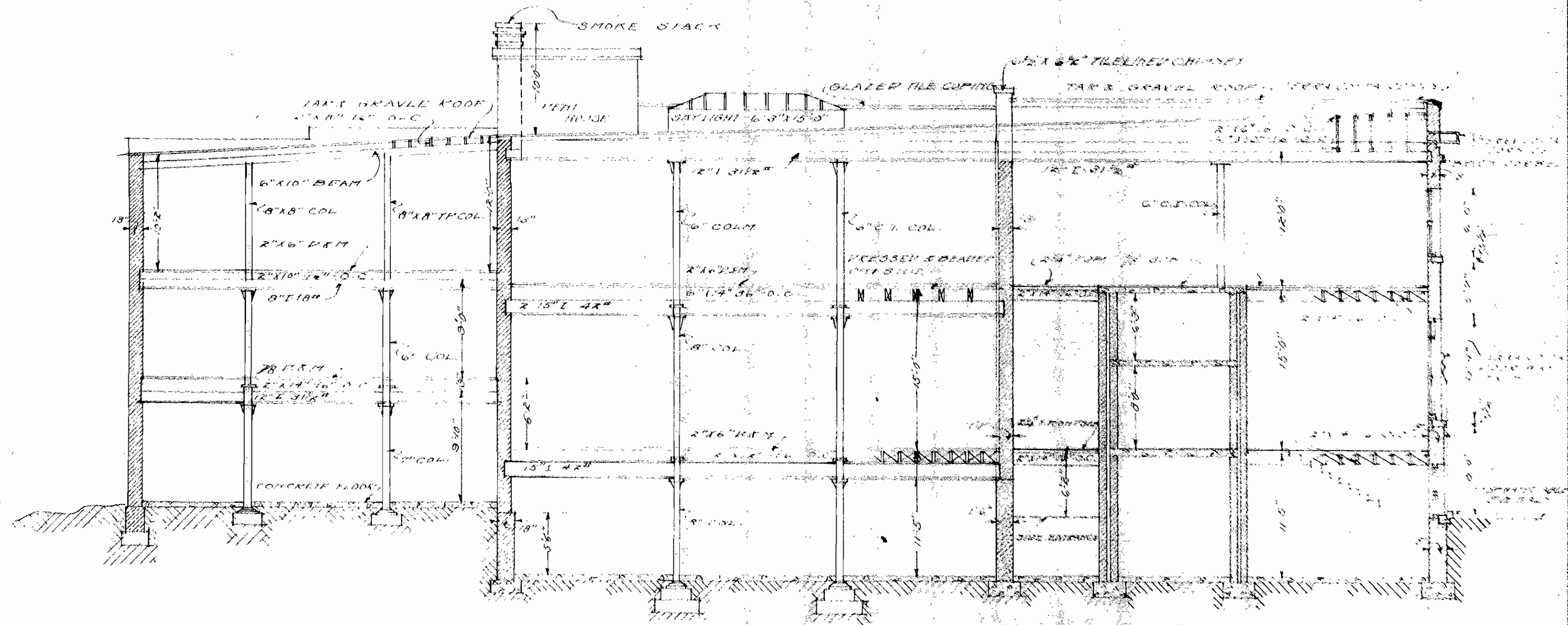
CROSS SECTION
