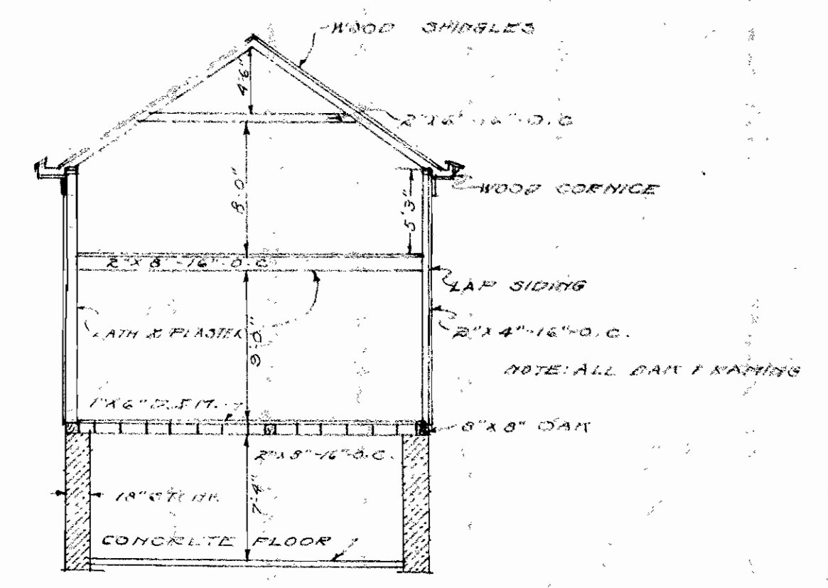
CROSS SECTION
