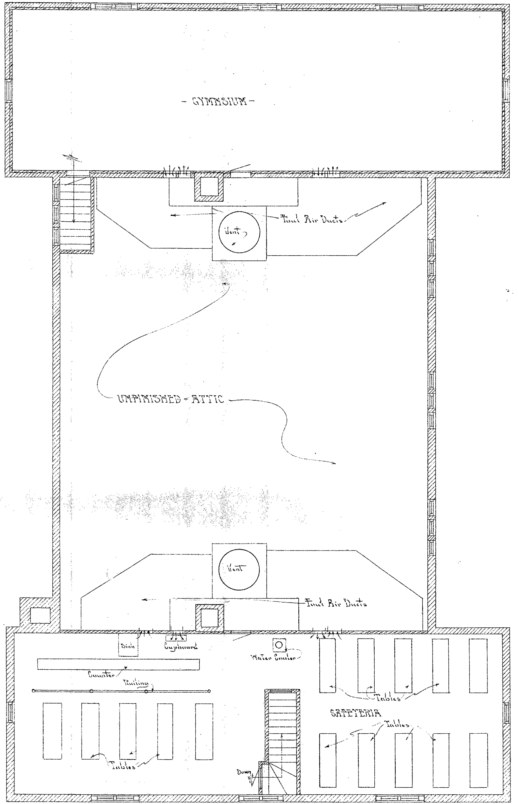
ATTIC - FLOOR - PLAN
